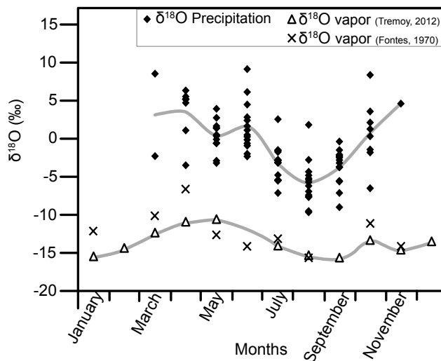
Figure 4. Isotopic composition of precipitations (black diamonds, data from GNIP, IAEA), and regional atmospheric vapor measured by Tremoy et al. (2012), triangles, and by Fontes et al. (1970a), black crosses. The grey lines represent the mean annual scenarii.
