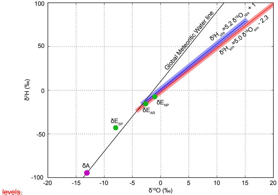
Figure 7. \delta^2\text{H} - \delta^{18}\text{O} cross plot showing the comparison between the observed evaporation line in Lake Chad in blue (according to (Fontes et al., 1970b)) and the simulated linear regression between \delta^2\text{H} and \delta^{18}\text{O} in Lake Chad in red. In addition, average isotopic compositions are shown for atmospheric moisture (purple) and simulated evaporates (green) above each pool (SP: southern pool, AR: archipelagos, and NP: Northern pool).
