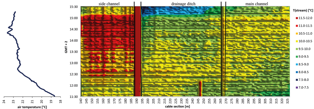
Figure 4. Air temperature (line diagram, left side) and surface water temperatures (colour plot, right side) of the Urbach on 3 September 2013. The x axis of the colour plot shows the sections of the fibre-optic cable in meters, the colours represent the surface water temperatures in °C. Thereby, each coloured line on the x axis, from cable section 140 to 327 m, represents one measurement. The y axis states the time of the measurements.
