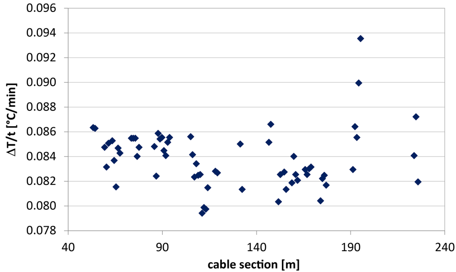
Figure 7. Cooling rates of cable sections with a temperature between 15.9 and 16.1 °C determined at 3 a.m. on 4 July 2014 in [°C min -1 ].
