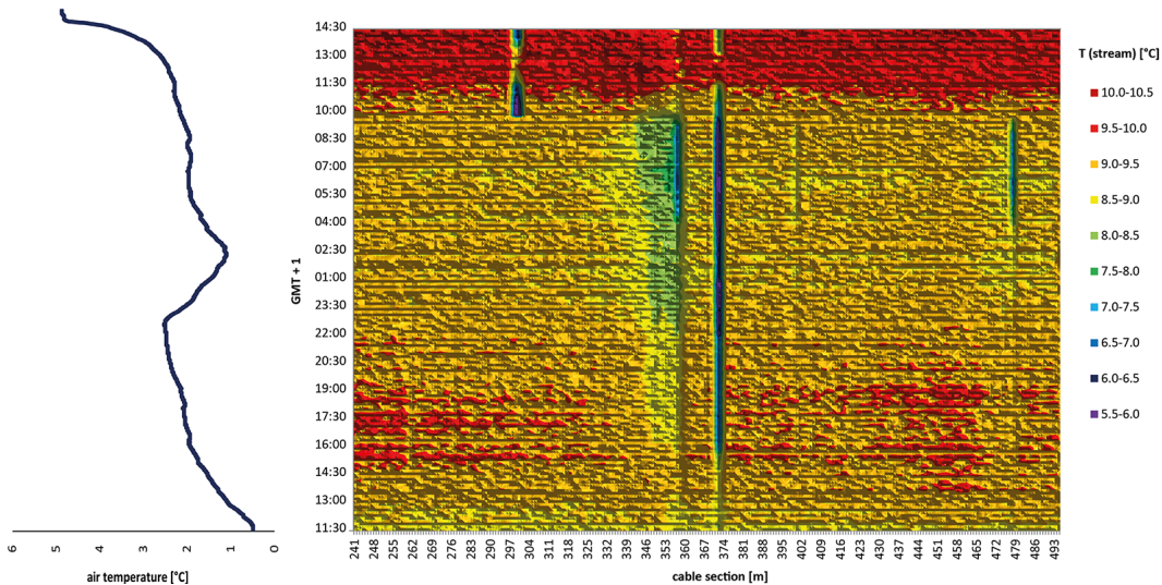
Figure 3. Air temperature (line diagram, left side) and surface water temperatures (colour plot, right side) of the Chriesbach after river restoration, on 28–29 November 2013. The x axis of the colour plot shows the sections of the fibre-optic cable in meters, the colours represent the surface water temperatures in °C. Each coloured line on the x axis, from cable section 241 to 493 m, represents one measurement. The y axis states the time of the measurements.
