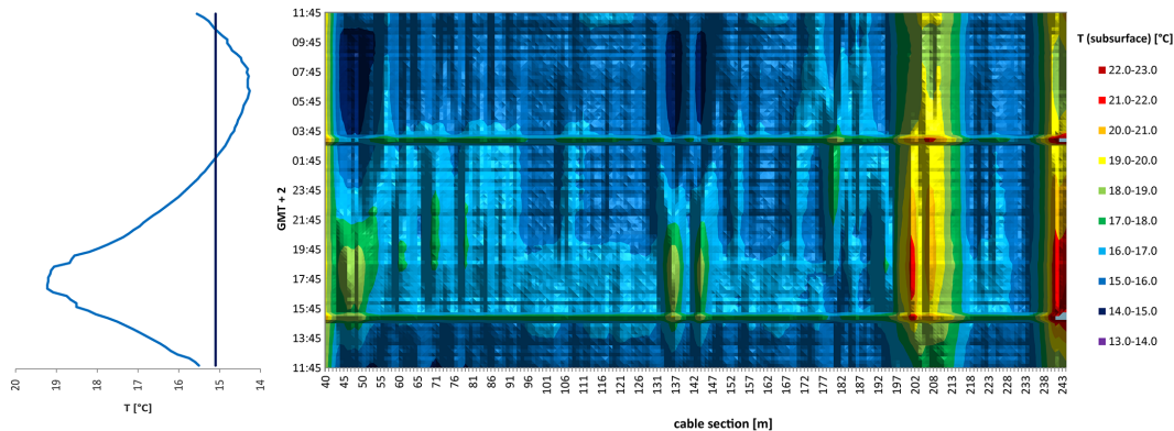
Figure 6. Surface water temperature (line diagram, left side) and streambed temperatures (colour plot, right side) in the Chriesbach streambed at about 0.4 m depth, as measured with a fibre-optic cable installed after river restoration on 3–4 July 2014. The x axis of the colour plot shows the section of the fibre-optic cable in meters, the colours represent the streambed temperatures in ^{\circ}\text{C} . Thereby, each coloured line on the x axis, from cable section 40 to 243 m, represents one measurement. The y axis states the time of the measurements.
