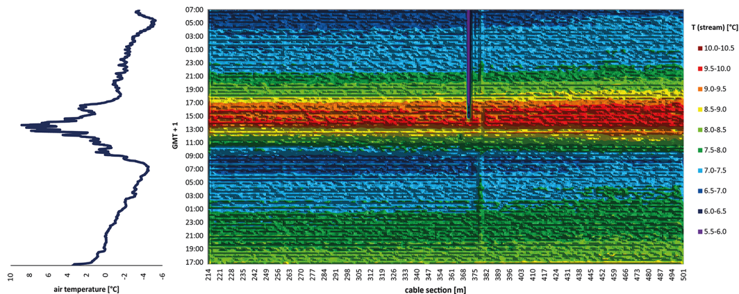
Figure 2. Air temperature (line diagram, left side) and surface water temperatures (colour plot, right side) of the Chriesbach before river restoration, on 13–15 March 2013. The x axis of the colour plot shows the sections of the fibre-optic cable in meters, the colours represent the surface water temperatures in °C. Thereby, each coloured line on the x axis, from cable section 214 to 501 m, represents one measurement. The y axis states the time of the measurements.
