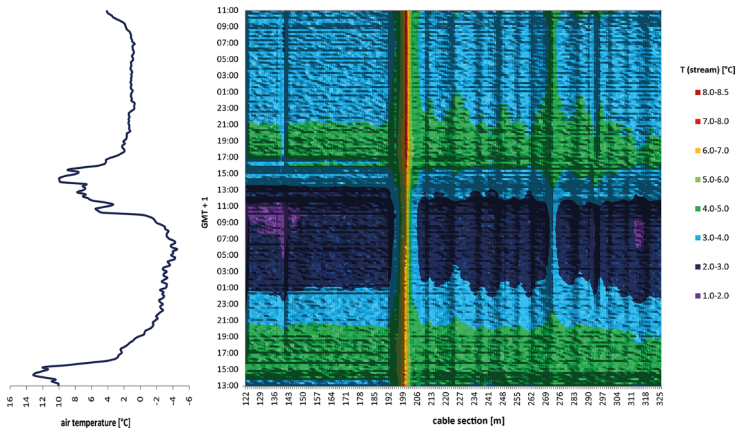
Figure 5. Air temperature (line diagram, left side) and surface water temperatures (colour plot, right side) of the Röthenbach on 17–19 February 2014. The x axis of the colour plot shows the sections of the fibre-optic cable in meters, the colours represent the surface water temperatures in °C. Thereby, each coloured line on the x axis, from cable section 140 to 325 m, represents one measurement. The y axis states the time of the measurements.
