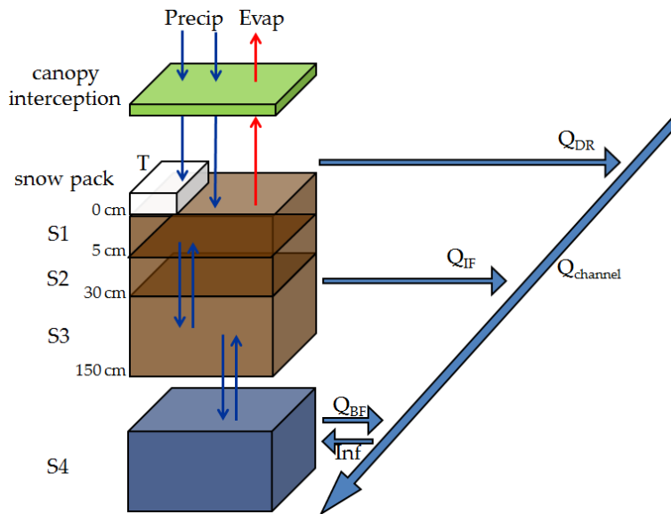
Figure 3. PCR-GLOBWB model structure, adapted from Van Beek et al. (2011). Symbols definition are as follows: Precip, precipitation; Evap, evaporation; T , Temperature; S1, first soil layer; S2, second soil layer; S3 third soil layer; S4, groundwater reservoir; Q_{channel} , total runoff; Q_{DR} , direct runoff; Q_{IF} , intermediate flow; Q_{BF} , baseflow and Inf , water flow from the river channel to the groundwater reservoir.
