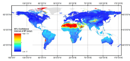
Figure 7: Confidence interval size for ET_LMM generated from 1000 bootstrapped datasets.
