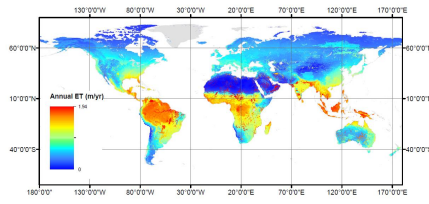
Figure 5. ET_LMM (m/yr) global annual actual ET projections. Potential vegetation with wetland overlay. Grey indicates areas permanently covered by ice or large lakes. ET_LMM maps for individual anthropogenic land covers are presented in Supplementary Information E.
