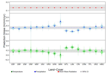
Figure 1: Linear mixed effect modelling slope by predictor. Slopes of two random effects (air temperature (green) and precipitation (blue)) and fixed slope (shortwave radiation (red)). The fixed effect is displayed by the dotted line, with the additional random effect shown by the dot. Lighter shading indicates the bootstrapped distribution, where the horizontal line is the mean of the bootstrapped distribution.
