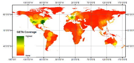
Figure 3: Global patterns of ET_OBS density for all LCs, as derived from the GETA 2.0 database. Circles represent the density of ET_OBS where "Highest" represents 1.26 points per 7.5 degree search radius and "None" represents zero data points per 7.5 degree search radius.
