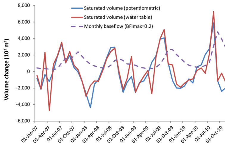
Figure 7. Monthly variations in saturated volumes for the catchment area with elevation <100 m for both the potentiometric and water table datasets and for monthly baseflow derived from Eckhardt analysis (using BFI_{max} value of 0.2).
