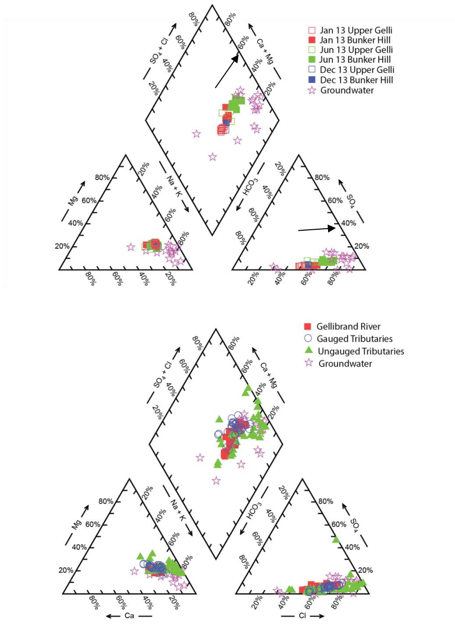
Figure 3. Piper diagrams showing temporal and spatial patterns in the chemistry of streamflow and groundwater. The top panel shows seasonal variations in composition of flow in the Gellibrand River at the upstream (Upper Gellibrand) and downstream (Bunker Hill) sites over three sampling trips. The internal arrows show direction of compositional change from upstream to downstream and also from summer to winter towards the general groundwater composition. The lower panel shows compositional differences across all sampling trips between Gellibrand River, gauged tributaries, ungauged tributaries and groundwater.
