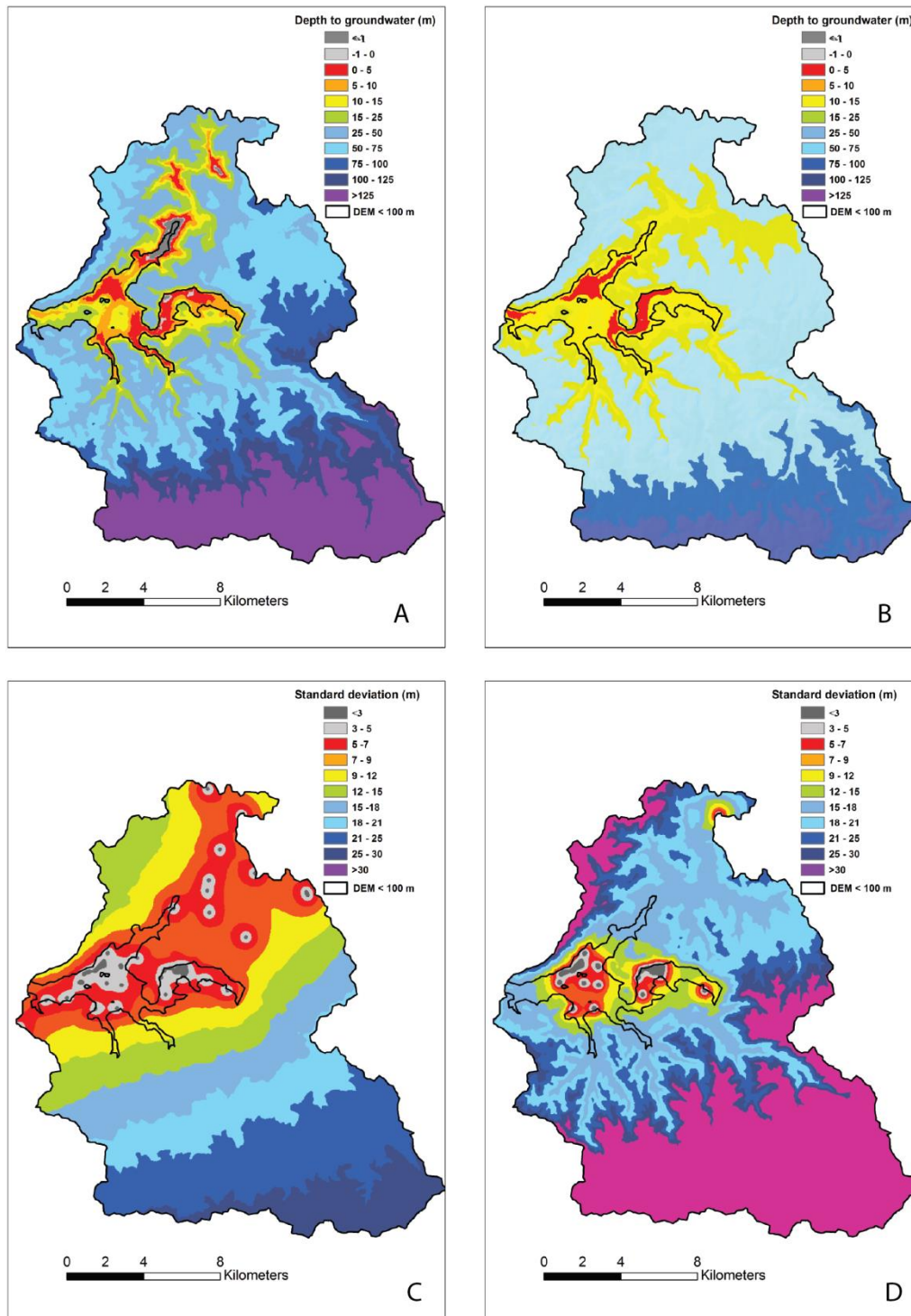
Figure 5. Depth to groundwater maps (A – ‘potentiometric surface’ (all bores), B – ‘water table’ (shallow bores)) and kriging standard deviation (C – potentiometric surface, D – water table) for 1 st September 2009. Areas of shallow or intersecting (artesian) groundwater are restricted to the Gellibrand River (centre) and Love Creek (north) valley floors.
