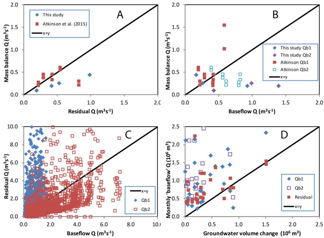
Figure 9. Scatter plots showing various estimates of baseflow and groundwater discharge. (a) Mass balance tracer estimates (from Atkinson et al. (2015) for 2011-2012 and mid-point of range shown in Table 1 for 2013) for groundwater discharge against the residual streamflow (Bunker Hill streamflow less upstream gauged streamflow). (b) Mass balance tracer estimates against the Eckhardt filter baseflow estimates (Qb1 uses a=0.988 and \text{BFI}_{\text{max}}=0.2 , Qb2 uses a=0.988 and \text{BFI}_{\text{max}}=0.6 ). (c) Residual discharge against Eckhardt filter baseflow timeseries for 2007-2013. (d) Saturated volume changes (using specific yield set 0.15, 0.30, 0.05 from Table 2) against residual flow and Eckhardt filter baseflow timeseries.
