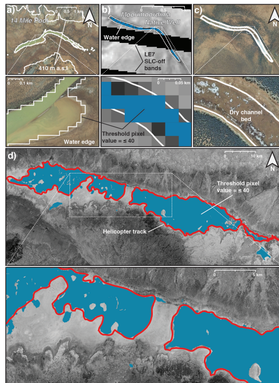
Fig. 2. Figure A1: Validation and groundtruthing of standing water on the Fortescue Marsh, including: a) standing water on the 14 Mile Pool extracted from Level 1T Landsat image (Jul 2010; solid white line =
