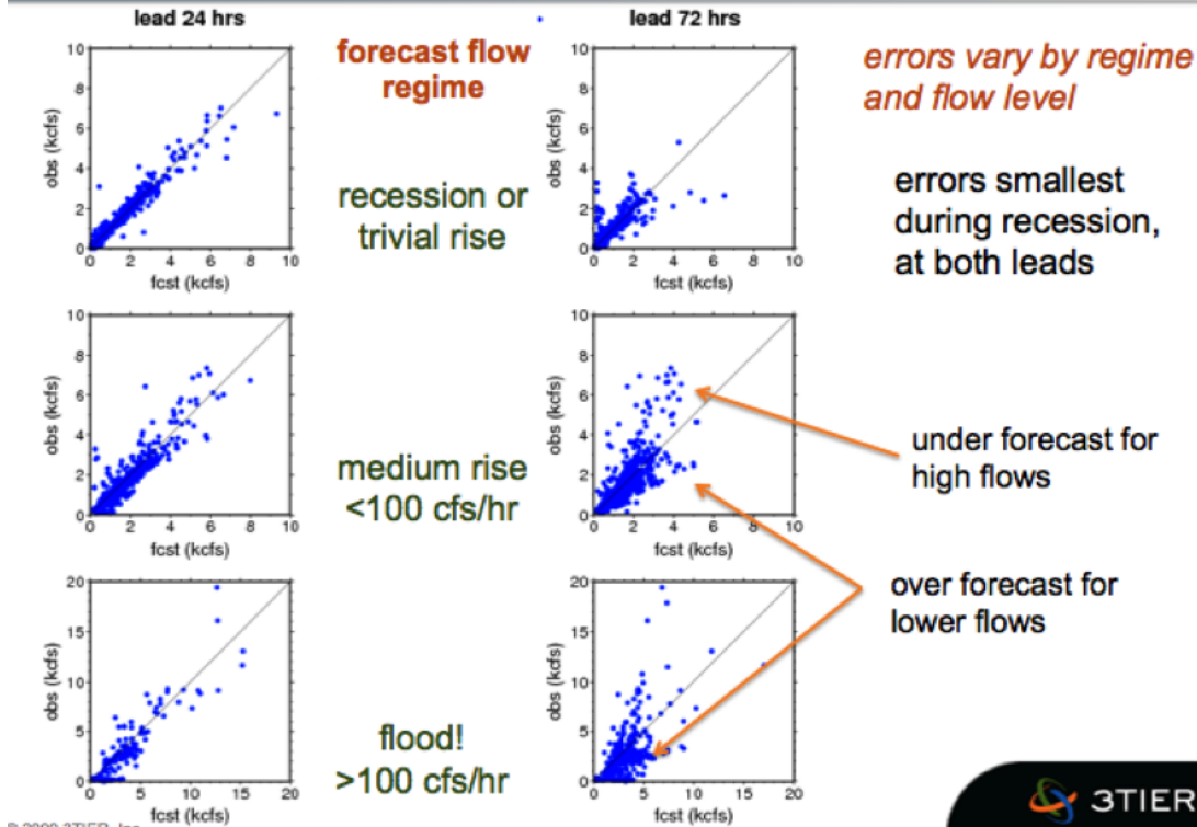
Fig. 2. Figure 2, Description of streamflow rise and lead time conditioning factor from Wood et al (2009)
