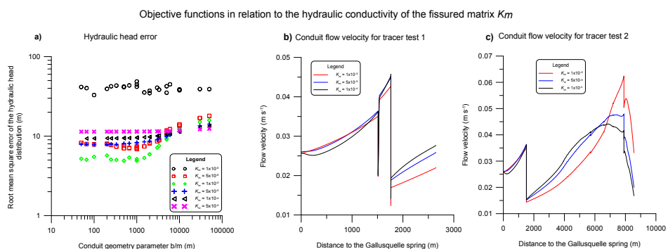
Fig. 1. Influence of the fissured matrix conductivity a) on the hydraulic head distribution in relation to the conduit geometry, b) and c) on the tracer velocities.
