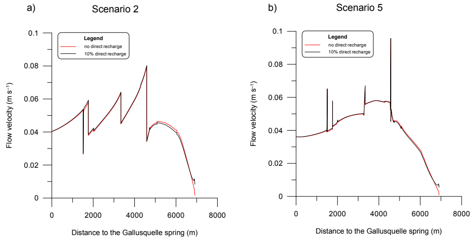
Fig. 2. Flow velocities inside the main conduit branch with and without direct recharge for the best-fit scenarios.
