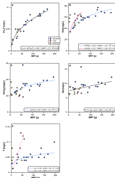
Figure 7. (a) Dissolved reactive phosphate ( \text{PO}_4\text{-P} ), (b) silica ( \text{SiO}_2 ), (c) bicarbonate ( \text{HCO}_3 ), (d) sodium ( \text{Na} ), and (e) fluoride ( \text{F} ) vs. mean residence time (MRT). The sample colour code for all graphs is shown in graph (a), and indicates water origin from the relevant geologic formation, as indicated by Hierarchical Cluster Analysis (HCA).
