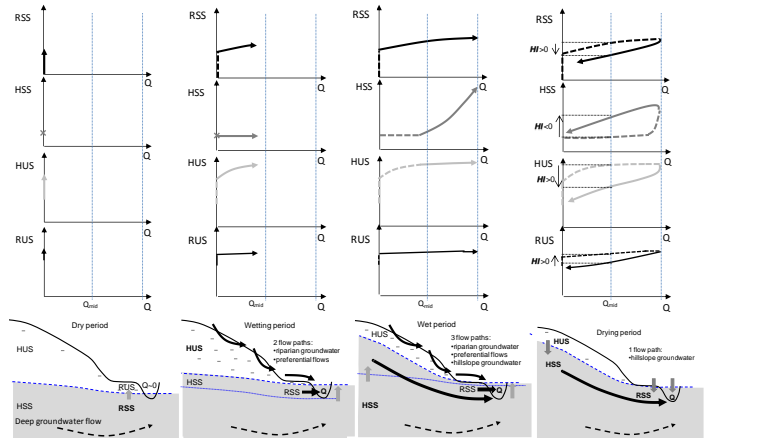
Figure 9: Conceptual scheme of successive mechanisms which explain the annual hysteresis between storages and stream flows. HUS: Hillslope unsaturated storage, HSS: hillslope saturated storage, RUS: riparian unsaturated storage, RSS: riparian saturated storage, Q: stream flow, bold characters indicate varying components, grey arrows indicate if the component is increasing or decreasing, black arrows indicate the water flow paths.
