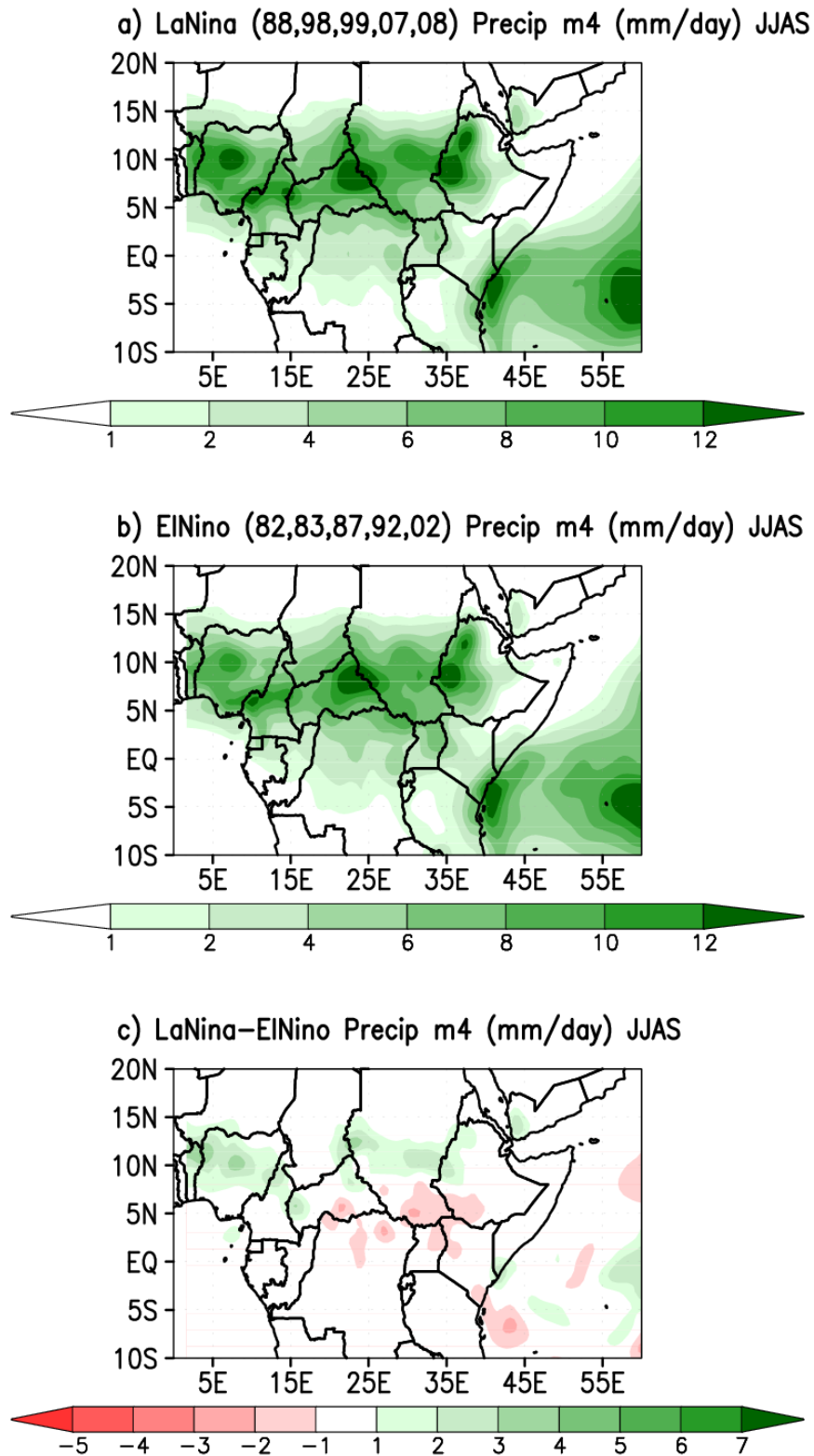
Figure A.4: The rainfall in North Africa during JJAS of member 4 and for (a) 5 La Niña years (88,98, 99, 07 and 08), (b) 5 El Niño years (82, 83, 87, 92 and 02), and (c) The difference between La Niña years and El Niño years.
