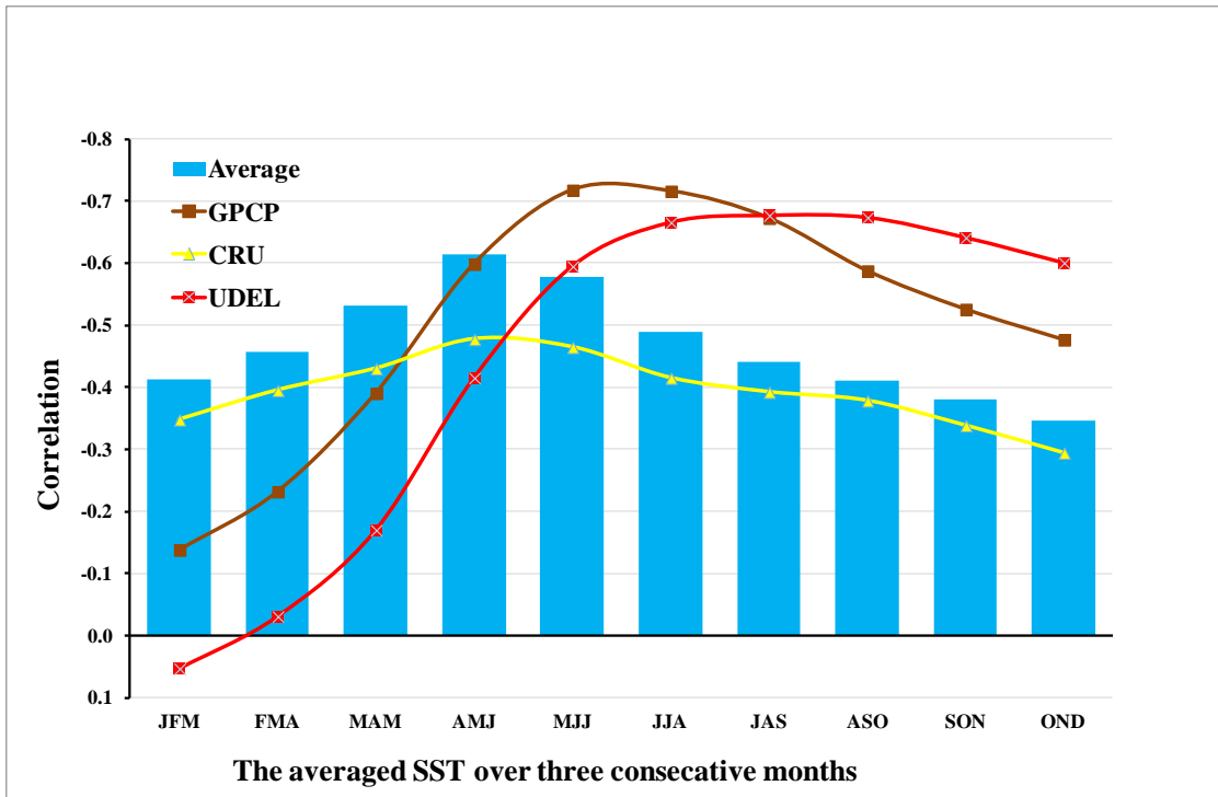
Fig. 10. Correlation between rainfall anomalies over the Ethiopian Highlands (Reg-TB ensemble average, GPCP, and CRU) and SST anomalies over the Pacific Ocean in the Niño 3.4 region.
