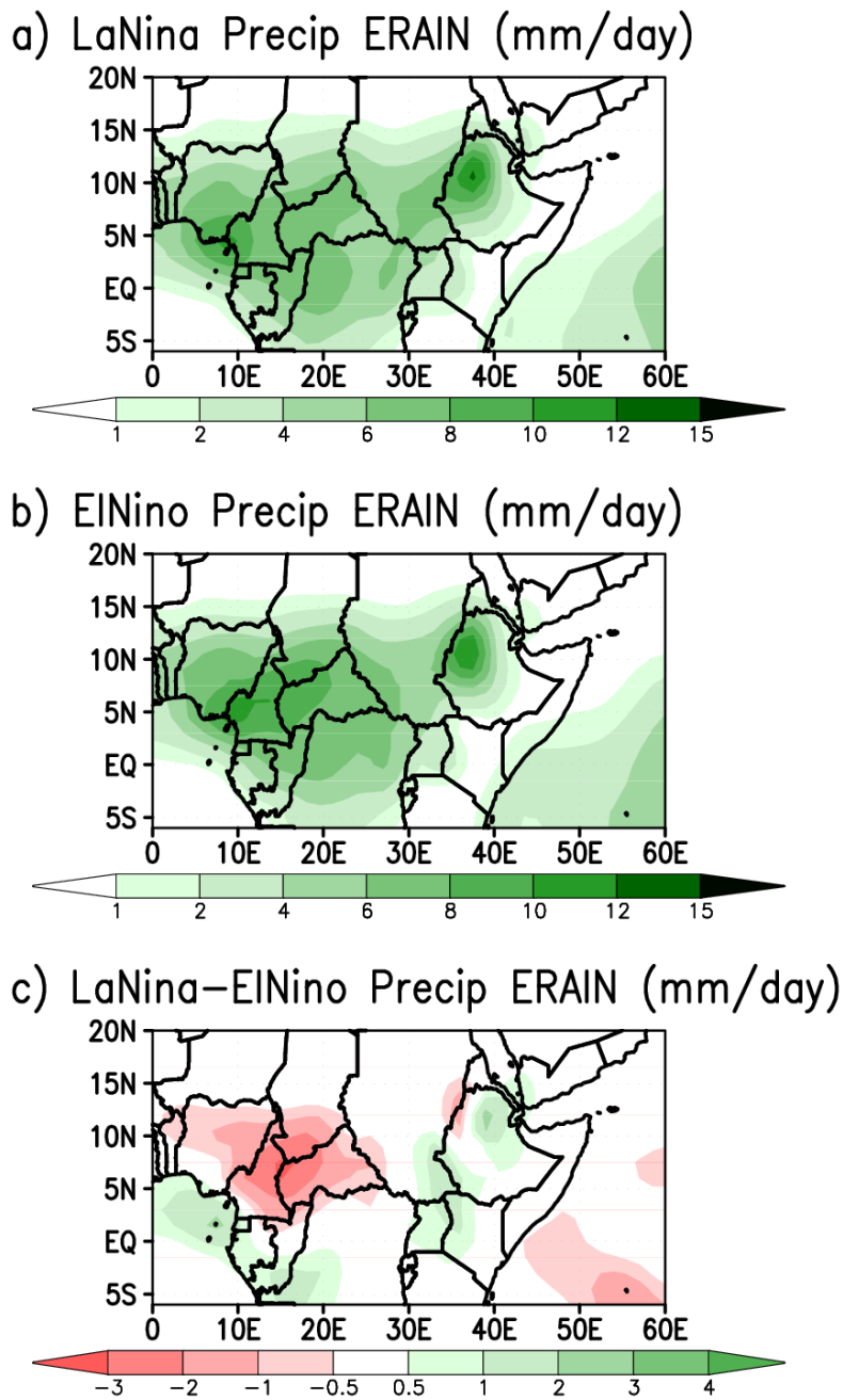
Fig. 9. ERA Interim JJAS rainfall for (a) 5 La Niña years (88,98, 99, 07 and 08), (b) 5 El Niño years (82, 83, 87, 92 and 02), and (c) The difference between La Niña years and El Niño years.
