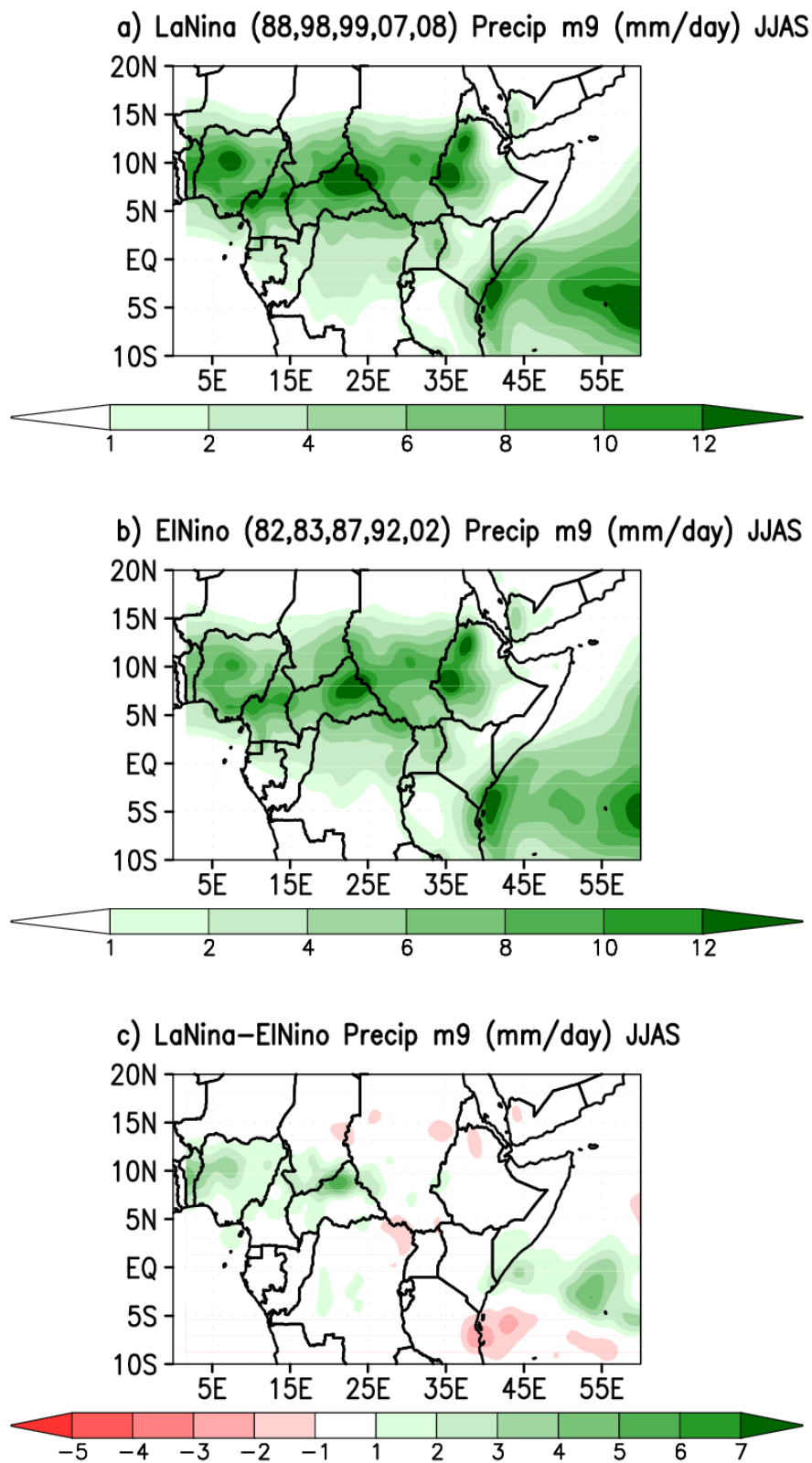
Figure A.9: The rainfall in North Africa during JJAS of member 9 and for (a) 5 La Niña years (88,98, 99, 07 and 08), (b) 5 El Niño years (82, 83, 87, 92 and 02), and (c) The difference between La Niña years and El Niño years.
