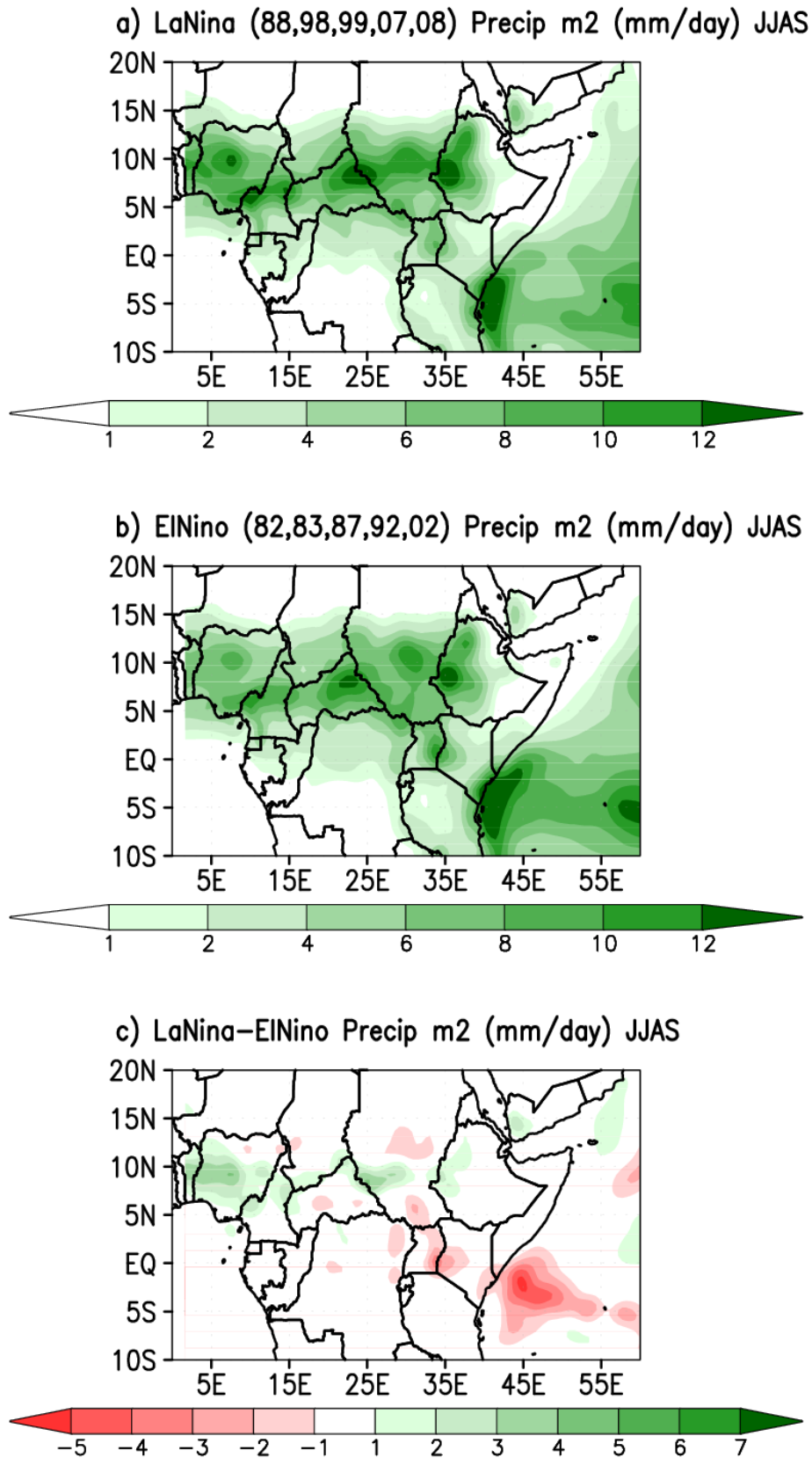
Figure A.2: The rainfall in North Africa during JJAS of member 2 and for (a) 5 La Niña years (88,98, 99, 07 and 08), (b) 5 El Niño years (82, 83, 87, 92 and 02), and (c) The difference between La Niña years and El Niño years.
