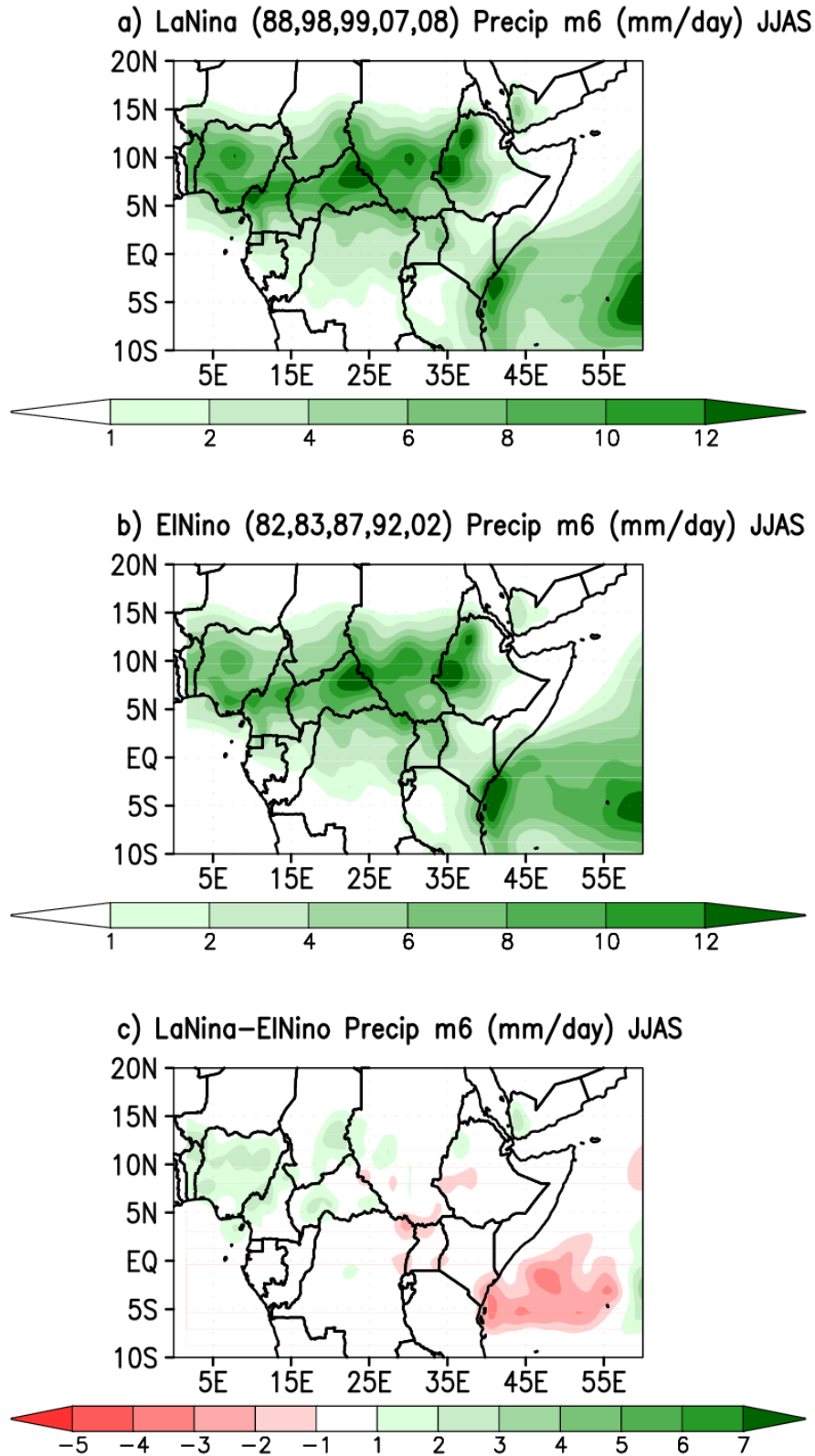
Figure A.6: The rainfall in North Africa during JJAS of member 6 and for (a) 5 La Niña years (88,98, 99, 07 and 08), (b) 5 El Niño years (82, 83, 87, 92 and 02), and (c) The difference between La Niña years and El Niño years.
