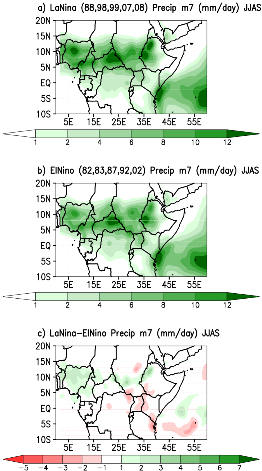
Figure A.7: The rainfall in North Africa during JJAS of member 7 and for (a) 5 La Niña years (88, 98, 99, 07 and 08), (b) 5 El Niño years (82, 83, 87, 92 and 02), and (c) The difference between La Niña years and El Niño years.
