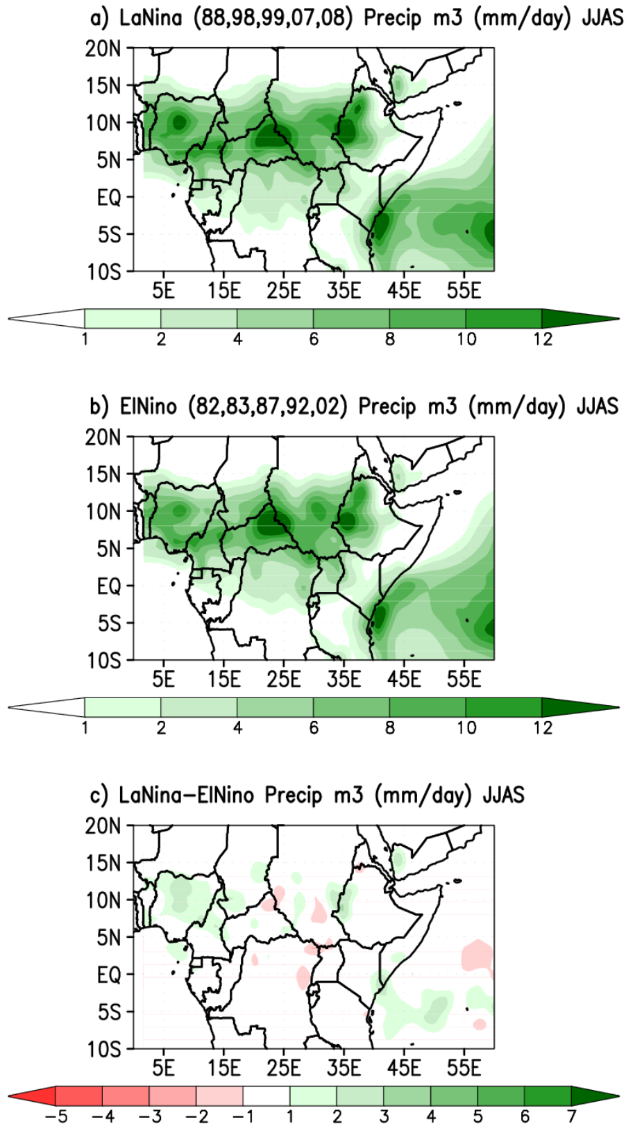
Figure A.3: The rainfall in North Africa during JJAS of member 3 and for (a) 5 La Niña years (88,98, 99, 07 and 08), (b) 5 El Niño years (82, 83, 87, 92 and 02), and (c) The difference between La Niña years and El Niño years.
