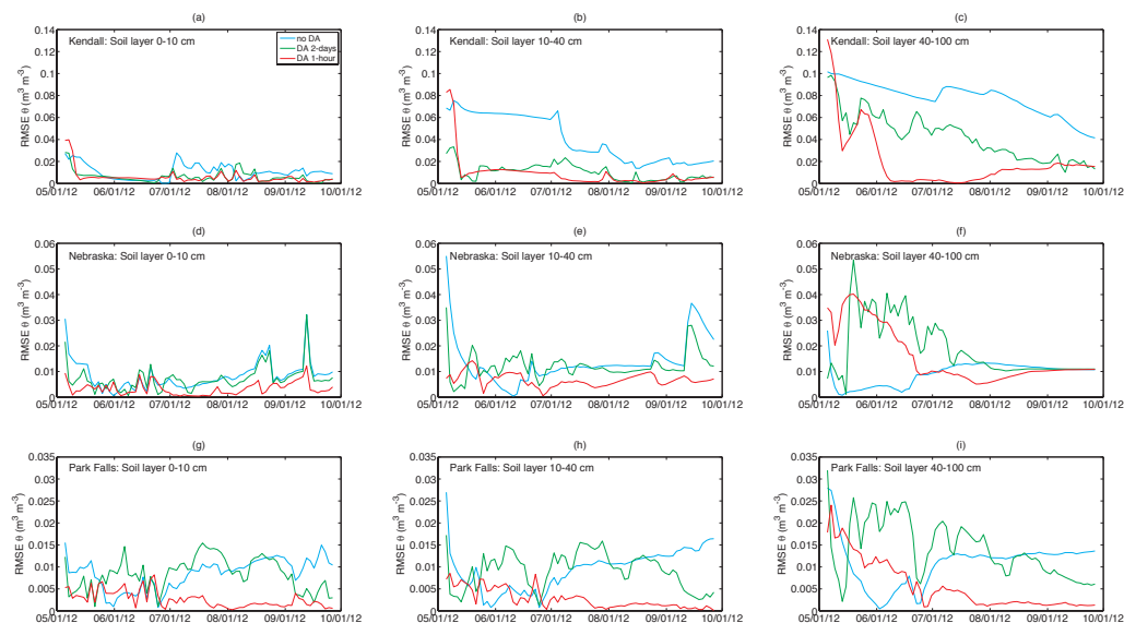
Figure 7. Comparison of Noah performance in representing soil moisture dynamics for the first three soil layers with respect to the true soil moisture state. The metric used is the Root-Mean-Squared-Error (RMSE) calculated over individual 2 day periods continuously. Results are shown for Noah without (no DA) and with data assimilation characterized by low- and high-frequency retrievals (respectively, DA 2-day and DA 1-hour). The ensemble mean of the prior distribution is used for all ensemble simulations.
