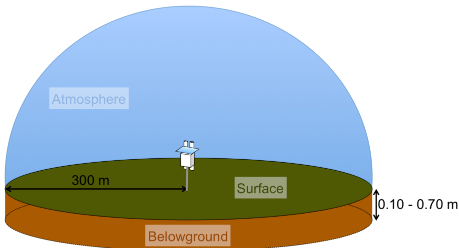
Figure 1. Schematic representation of the effective measurement volume for the cosmic-ray soil moisture sensor. The effective depth depicted in the figure refers to the overall range in the sensor (Zreda et al., 2008). Notice the effective depth estimated for the synthetic experiments in this study varies approximately between 12 and 20 cm (refer to text).
