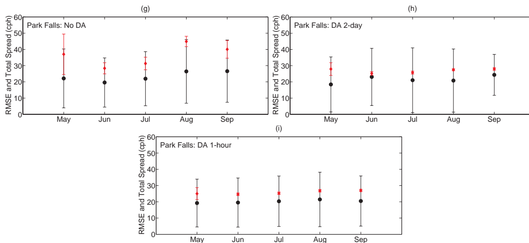
Figure 3. Monthly-average Root-Mean-Squared-Error (RMSE) calculated for the ensemble mean relative to the observations (black circles) in comparison to the monthly-average total ensemble spread (red diamonds) defined as the square root of the total variance (i.e., the sum of the ensemble variance plus the observational error variance). The error bars represent one standard deviation. The ensemble mean of the prior distribution is used for all ensemble simulations.
