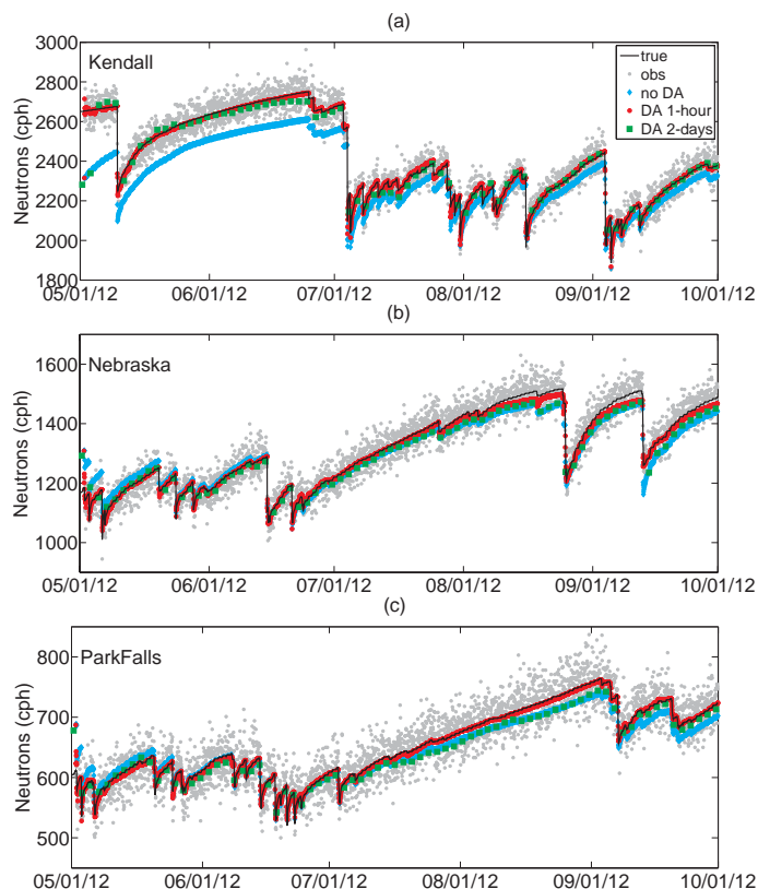
Figure 2. Equivalent neutron intensity (counts per hour – cph) simulated by Noah coupled to COSMIC without (no DA) and with data assimilation characterized by low- and high-frequency retrievals (respectively, DA 2-day and DA 1-hour) compared to synthetic observations (obs) and true intensities. The ensemble mean of the prior distribution is shown for all ensemble simulations.
