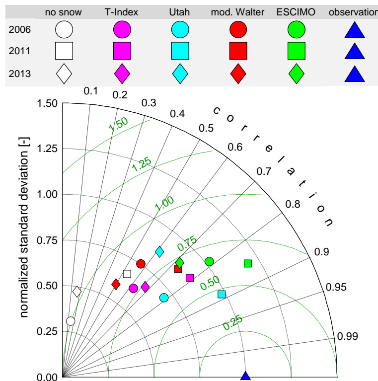
Fig. 1. Taylor plot including point scale simulations for three winter seasons. All simulation runs are based on modelled WRF precipitation.
