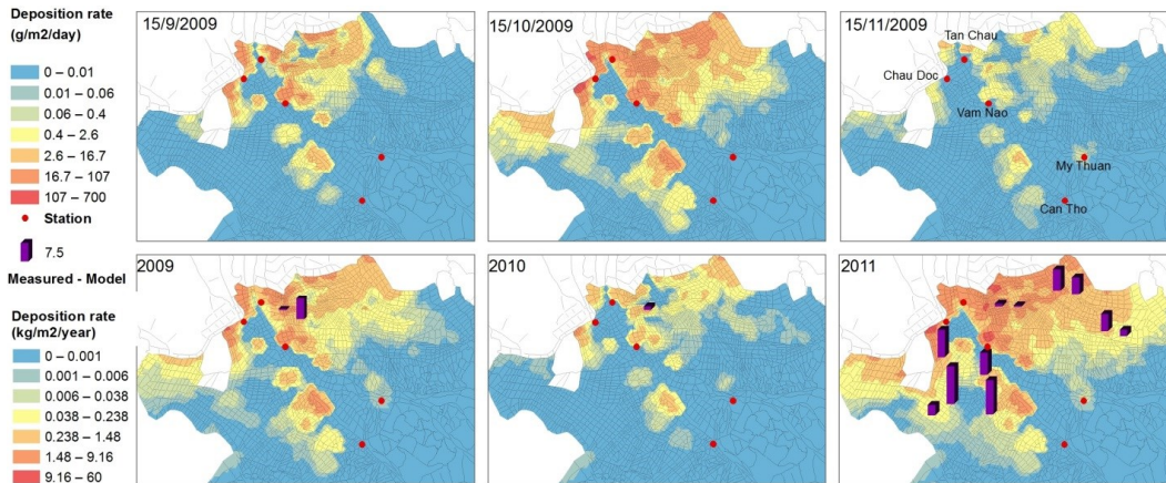
Fig. 9. Map of sedimentation in the VMD floodplains. Top panels: sediment deposition rate ( \text{g m}^{-2} \text{day}^{-1} ) during the period of compartment opening (left panel), during flood peak discharge (center panel) and during the period of compartment closing (right panel). Bottom panels: cumulative sediment deposition ( \text{kg m}^{-2} \text{yr}^{-1} ) in 2009, 2010 and 2011. The bars show the differences of cumulative sediment deposition between measurements and simulation.
