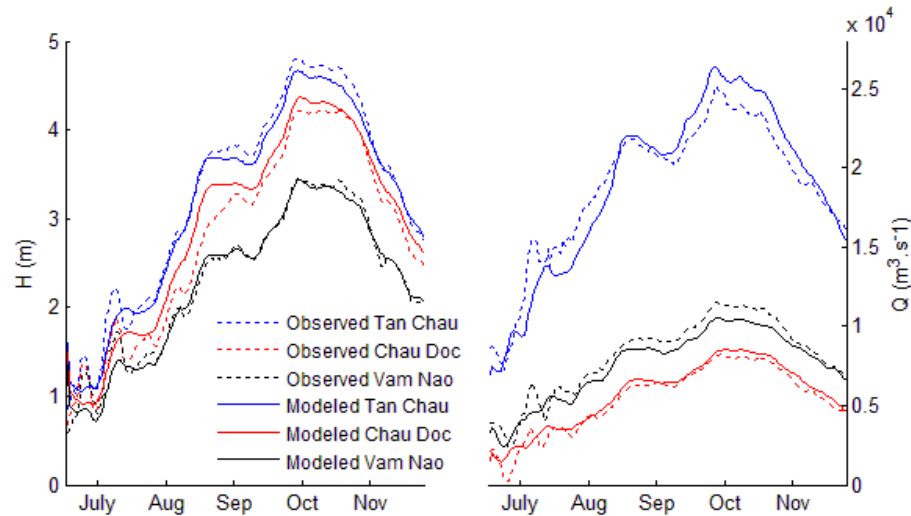
Fig. 4a. Comparison of measurements and simulation results at stations Tan Chau, Chau Doc and Vam Nao for 2011: daily water levels (left panel), daily discharges (right panel).
