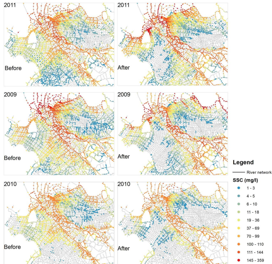
Fig. 6. SSC distribution in the VMD for three floods: SSC distribution before (left panels) and after (right panels) sluice gate opening.
