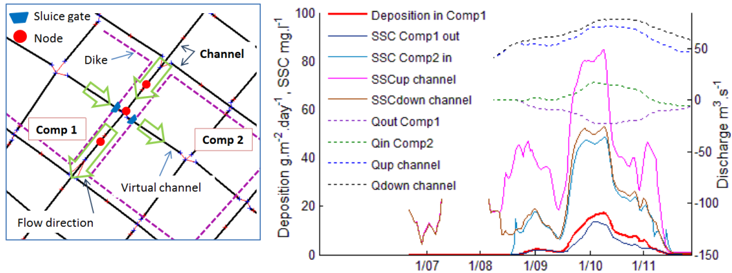
Fig. 8. Flow direction in channels and two nearby compartments (left panel). Discharge and sediment dynamics between a channel and two nearby compartments and sediment deposition in compartment 1 for 2011 (right panel).
