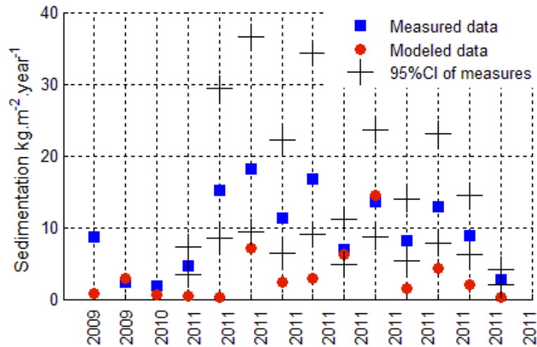
Fig. 4c. Comparison of measured and simulated sedimentation (2 locations in 2009, 1 location in 2010, 11 locations in 2011).
