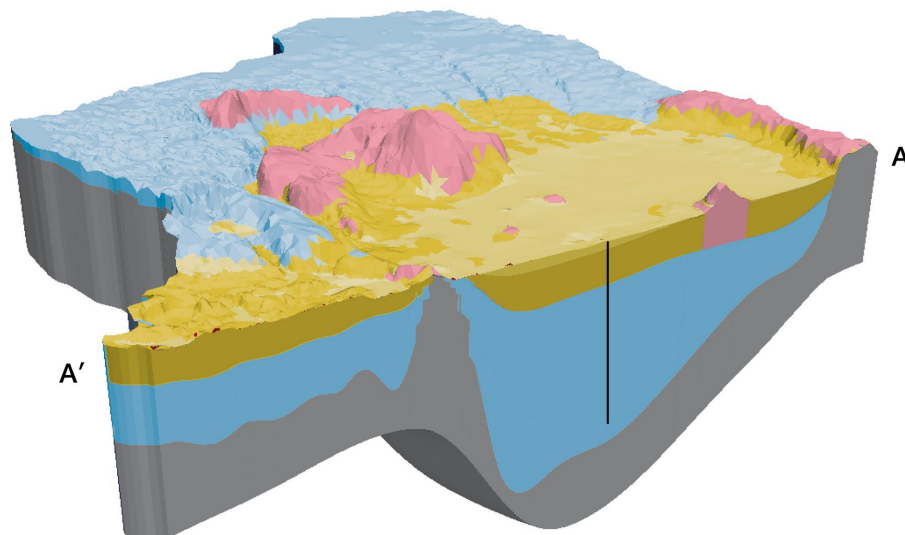
Figure 2. Three-dimensional geological model of the Lake Rotorua catchment area (from White et al., 2007). The location of the vertical cut-away face A'–A is shown in Fig. 1. The vertical exaggeration is 5×, with a 1 km vertical scale bar shown in the centre. The colour scheme is similar to that in Fig. 1 (bottom to top): Pre-Mamaku formations (grey), Mamaku Plateau Formation (light blue), sediment formation (dark yellow), lava domes (red) and Holocene alluvial deposits (light yellow).
