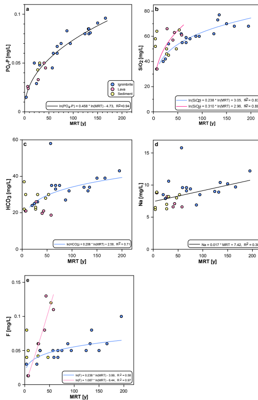
Figure 7. (a) Dissolved reactive phosphate ( \text{PO}_4\text{-P} ), (b) silica ( \text{SiO}_2 ), (c) bicarbonate ( \text{HCO}_3 ), (d) sodium (Na), and (e) fluoride (F) vs. mean residence time (MRT). The sample colour code for all graphs is shown in graph (a), and indicates water origin from the relevant geologic formation, as indicated by Hierarchical Cluster Analysis (HCA).
