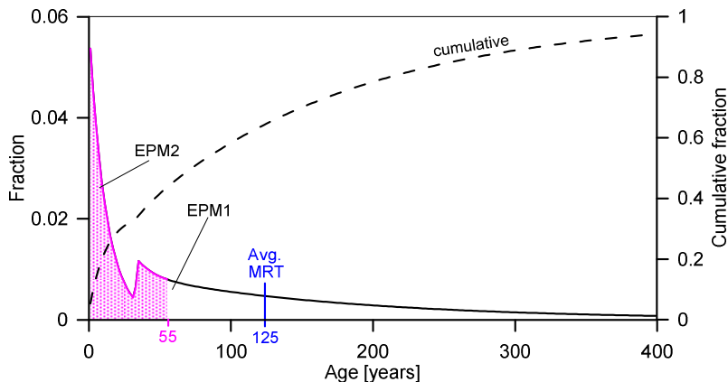
Figure 10. Age distribution for Hamurana Stream (at inflow into Lake Rotorua). The red shaded area indicates the fraction of water that was recharged after land-use intensification. EPM1 and EPM2 are exponential piston flow models.
