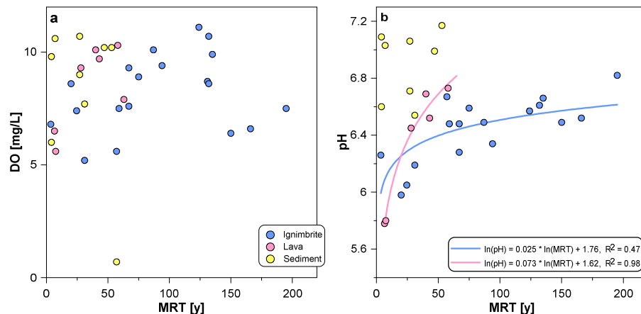
Figure 6. (a) Dissolved Oxygen (DO) and (b) pH vs. mean residence time (MRT). The colour codes of the samples indicate water from the relevant geologic formation, as indicated by Hierarchical Cluster Analysis (HCA).
