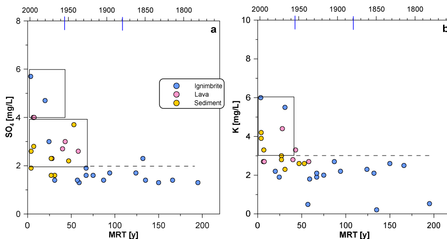
Figure 9. (a) Sulphate ( SO_4 ) and (b) potassium (K) vs. mean residence time (MRT). The sample colour code indicates water origin from the relevant geologic formation, as indicated by Hierarchical Cluster Analysis (HCA). The upper axis indicates calendar year.
