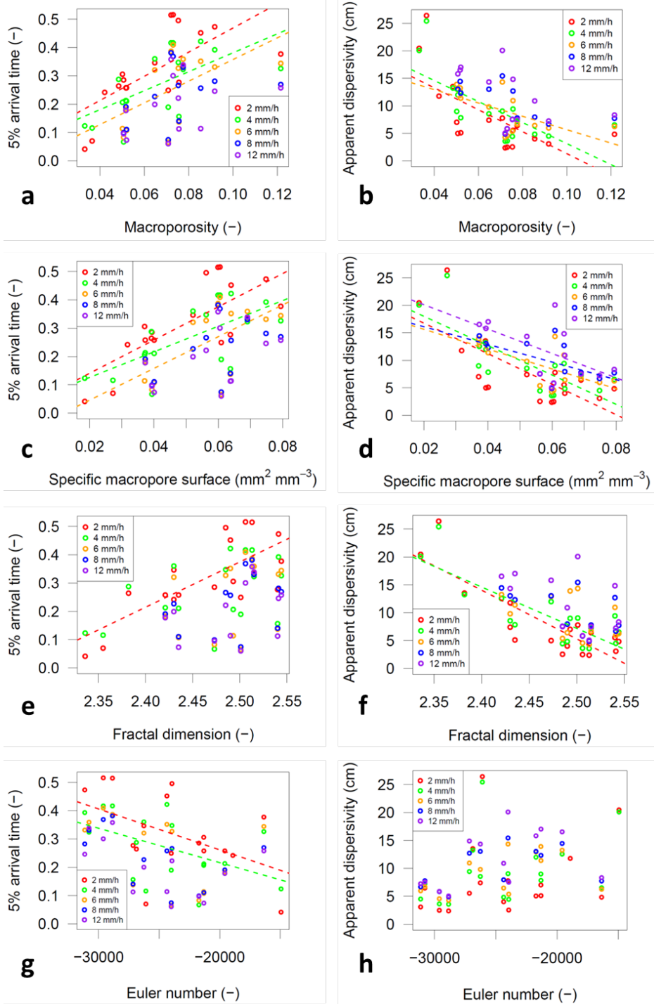
Figure 8. Relationship between macropore characteristics and measures of preferential transport for the four soils. Linear regression lines (dashed) were drawn if the slope was significantly ( p \leq 0.05 ) different from zero.
