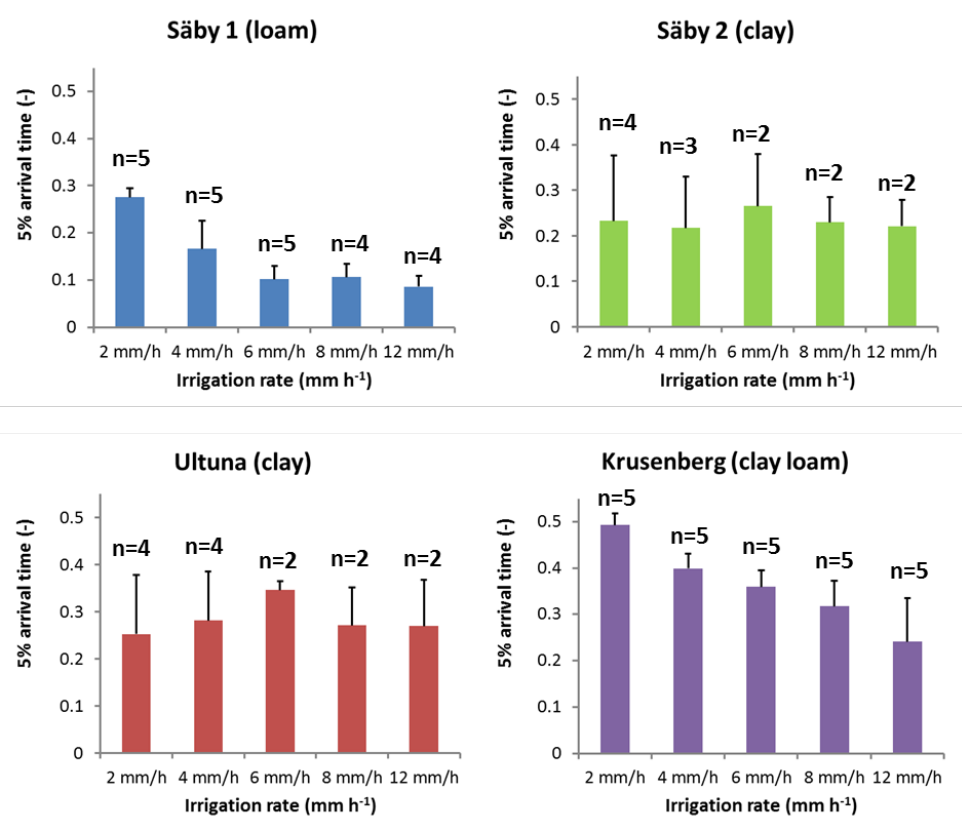
4 Figure 7. Mean 5% arrival times for the four soils. The number of breakthrough curves, n, was smaller 5 at higher irrigation rates due to ponding. Error bars indicate 1 standard deviation.
