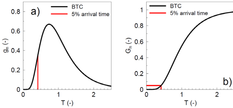
Figure 1. Illustration of the normalised 5% arrival time, p_{0.05} . Panel a) shows the travel-time probability density function, g_n , where the area to the left of the 5% arrival time equals 5% of the total area under the curve and panel b) shows the corresponding cumulative distribution function of the travel times, G_n . Both curves are plotted against the number of effective pore volumes drained ( T ).
