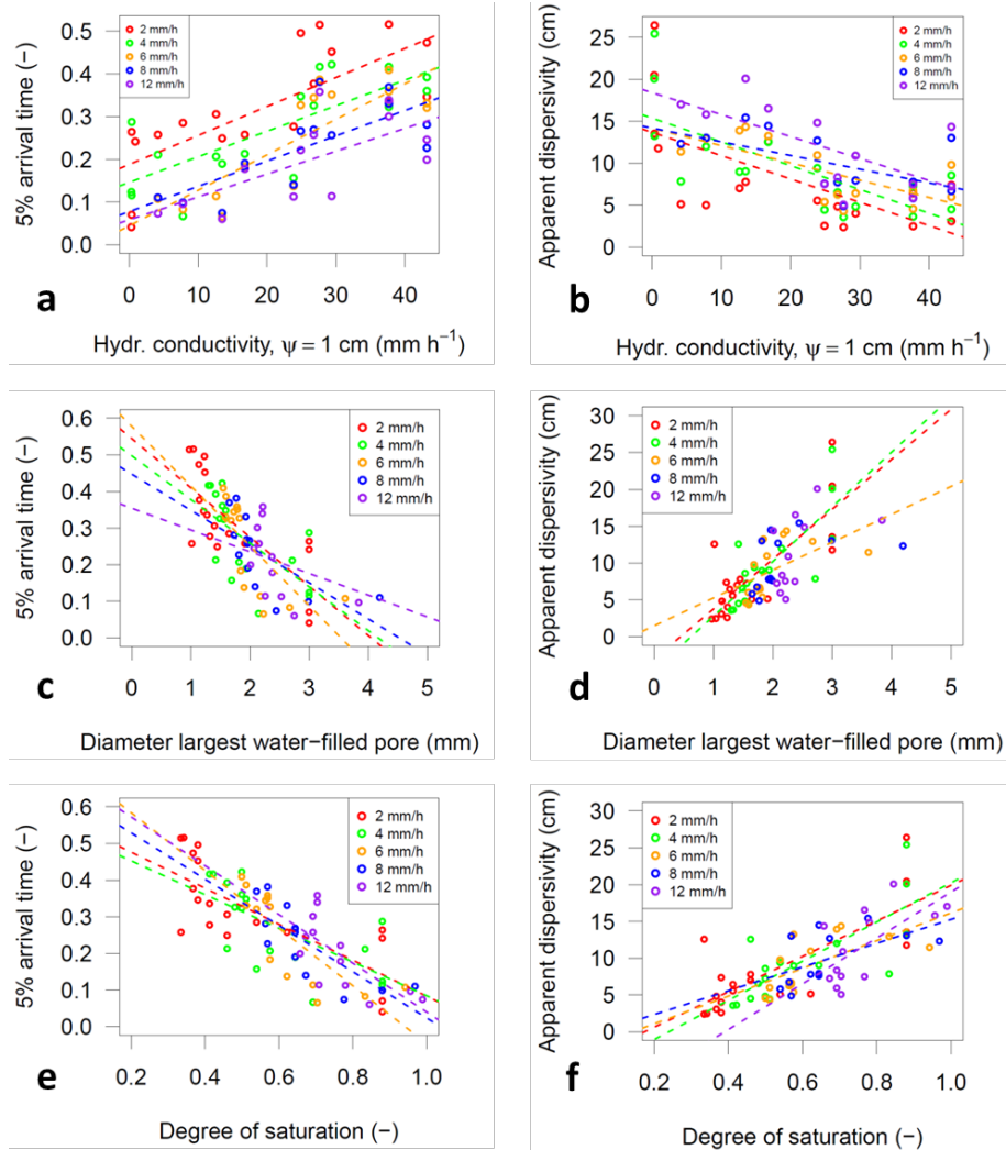
4 Figure 10. Relationship between hydraulic conductivity at \psi = 1 cm, the diameter of the largest 5 water-filled pore, the degree of saturation in the macropores and measures of preferential transport 6 for the four soils. Linear regression lines (dashed) were drawn if the slope was significantly ( p \leq 0.05 ) 7 different from zero.
