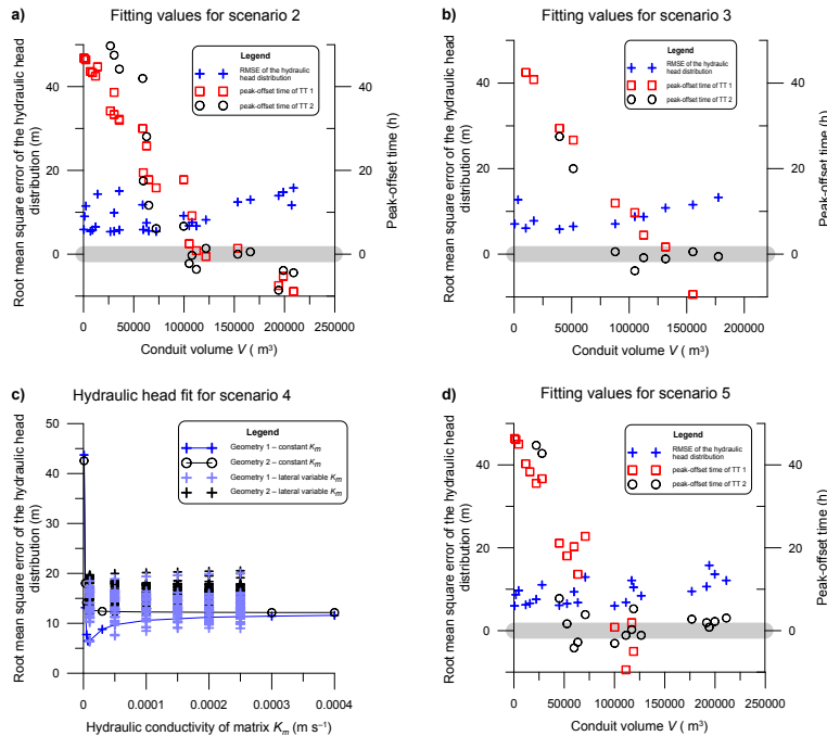
Figure 6. Calibrated values for the simulated scenarios. For scenarios 2, 3 and 5 (a, b and d) hydraulic head fit and the peak-offset times of both tracer tests (referred to as TT1 and TT2) are shown in relation to conduit volume. The thick grey bar marks the target value of zero. For scenario 4 (c) the root mean square error of the hydraulic heads is given for two different conduit geometries in relation to the hydraulic conductivity of the fissured matrix K_m . For the version with laterally variable matrix conductivity the axis shows as an example the hydraulic conductivity of the north-western part. The parameters for the two geometries are given in Table 3.
