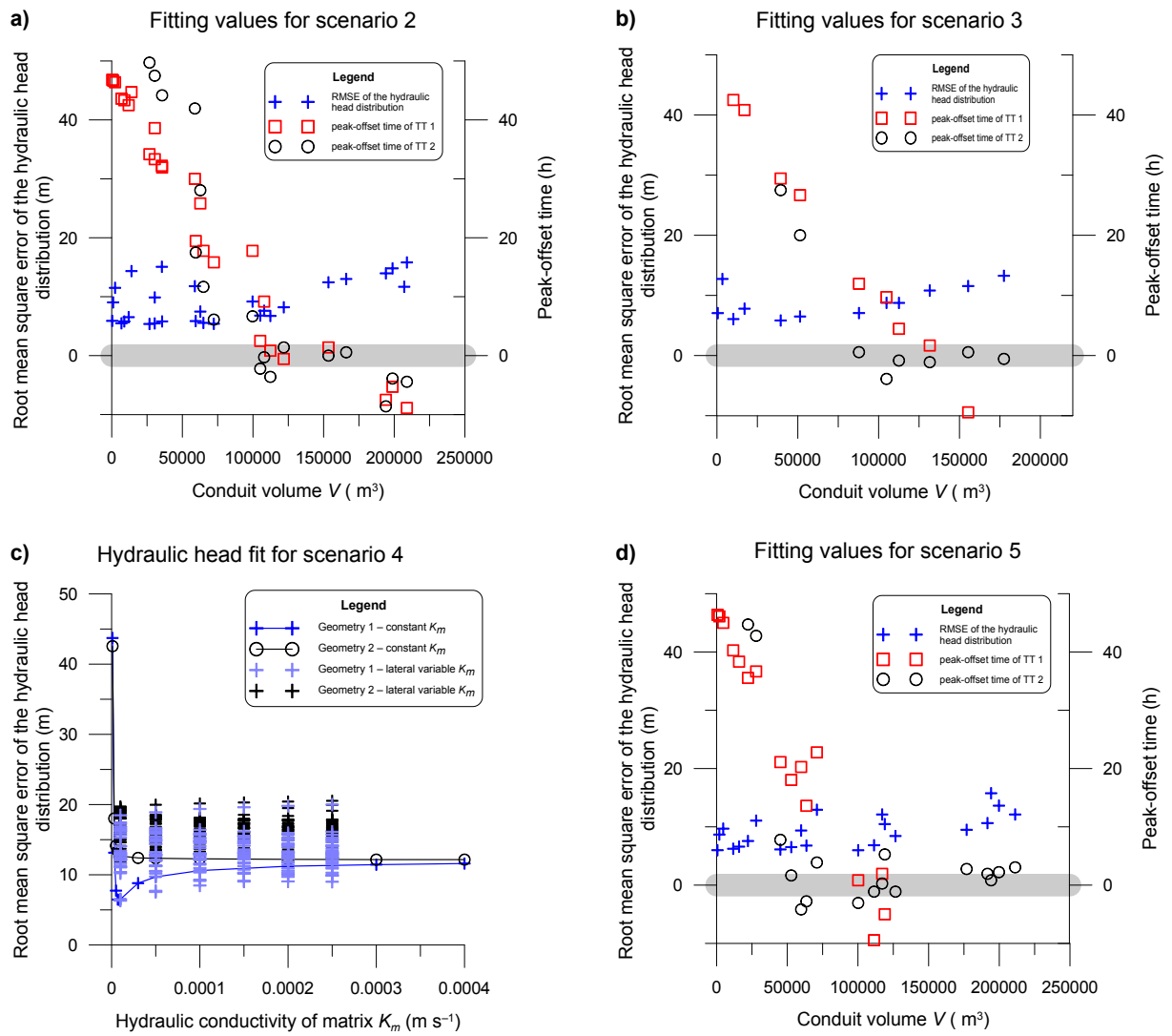
1 2 Figure 7. Calibrated values for the simulated scenarios. For scenarios 2, 3 and 5 (Fig. a, b and 3 d) hydraulic head fit and the peak-offset times of both tracer tests (referred to as TT 1 and 4 TT2) are shown in relation to conduit volume. The thick grey bar marks the target value of 5 zero. For scenario 4 (Fig. c) the root mean square error of the hydraulic heads is given for two 6 different conduit geometries in relation to the hydraulic conductivity of the fissured matrix 7 K_m . For the version with laterally variable matrix conductivity the axis shows as an example 8 the hydraulic conductivity of the north-western part. The parameters for the two geometries 9 are given in Table 3.
