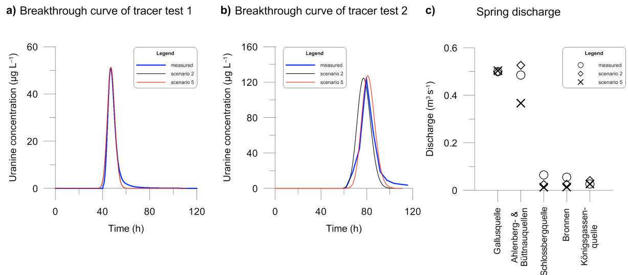
2 Figure 10. Comparison of the best-fit simulations with field data for scenarios 2 and 5. a) 3 breakthrough curve of tracer test 1, b) breakthrough curve of tracer test 2, c) spring discharge.
