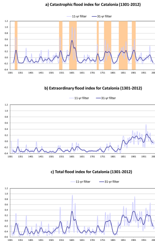
Figure 4. Temporal evolution of catastrophic (a), extraordinary (b) and total (c) flood index series for Catalonia (1301–2012). Data are smoothed by low-pass Gaussian filters of 31 and 11 yr. Anomalous periods of high catastrophic flood frequency are highlighted.
