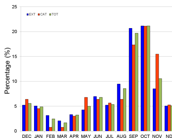
Figure 3. Temporal distribution of historical floods in Catalonia (1301–2012). Extraordinary (EXT), catastrophic (CAT) and total (TOT = EXT + CAT) floods. ND indicates floods with an unknown exact date.
