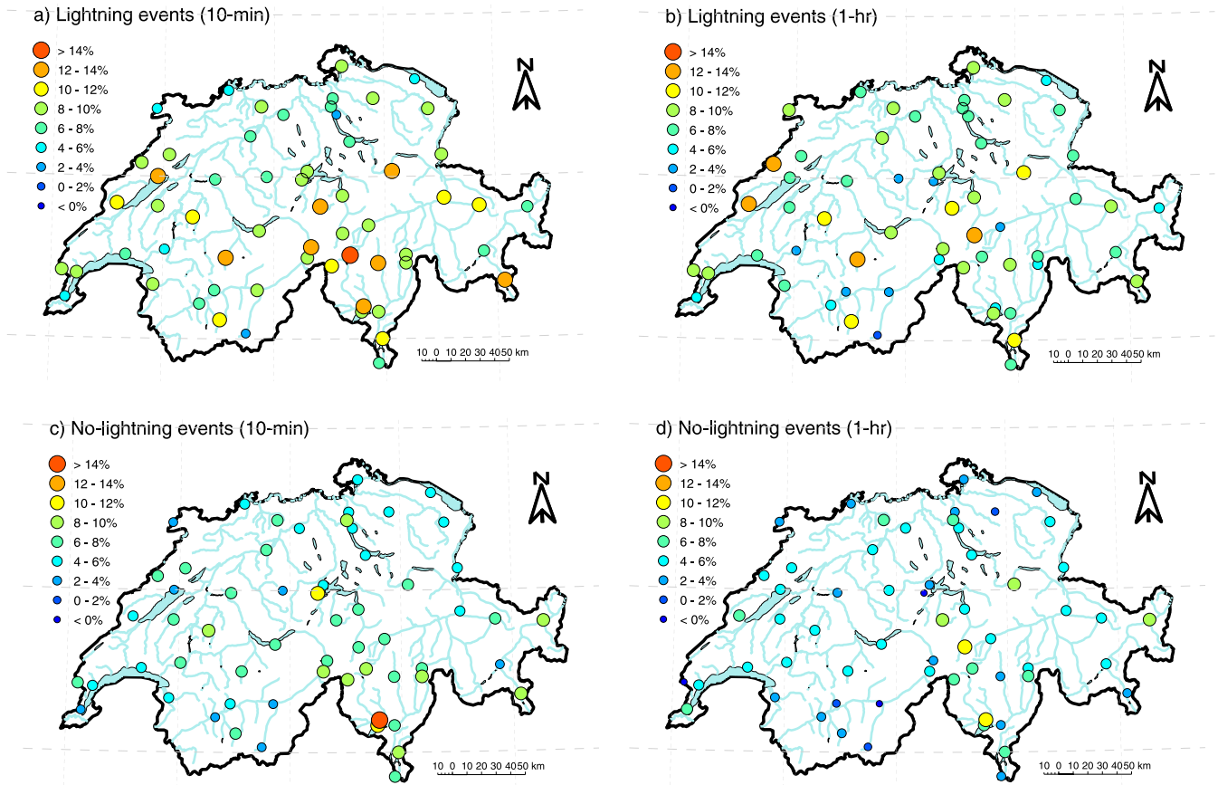
Figure 8. Spatial maps of scaling slopes for lightning events at the a) 10-min and b) 1-hr resolution; and no-lightning events at the c) 10-min and d) 1-hr resolution for the 95th percentile estimated with the quantile regression method. The color and size of the legend markers indicate the scaling slope magnitude in \% \text{ } ^\circ\text{C}^{-1} . The same figure for the temperature binning method is the Supplementary materials.
