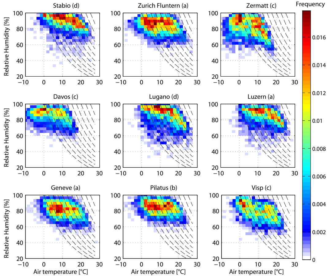
Figure 9. Relative frequency of mean daily relative humidity as a function of mean daily air temperature for wet days (precipitation larger than 1 \text{ mm day}^{-1} ) at nine representative stations in the four regions in our dataset: (a) Plateau, (b) pre-Alps, (c) Alps, (d) Tessin. Constant vapor pressure relations are shown with dashed lines.
