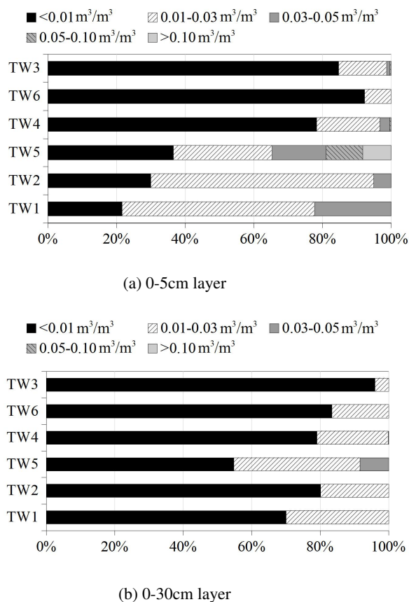
Fig. 6: Absolute water content difference distribution between the developed model and TEC for each climatic case study
