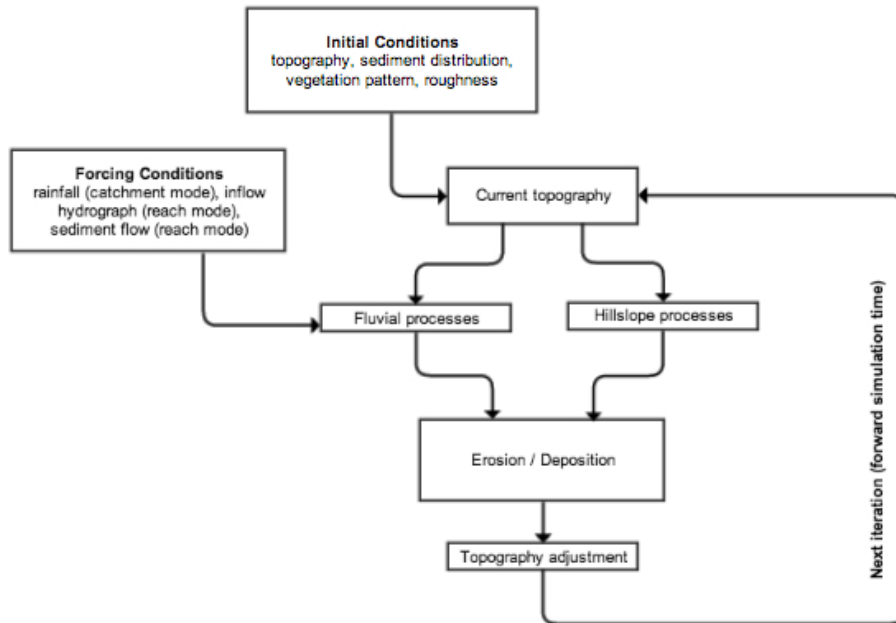
Fig. 2. Schematic of CAESAR's operation.
