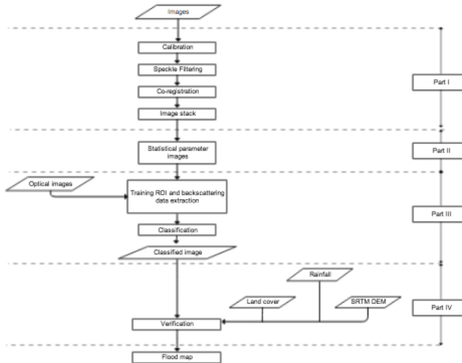
Fig. 9. Flow chart of the flooded area extraction.
