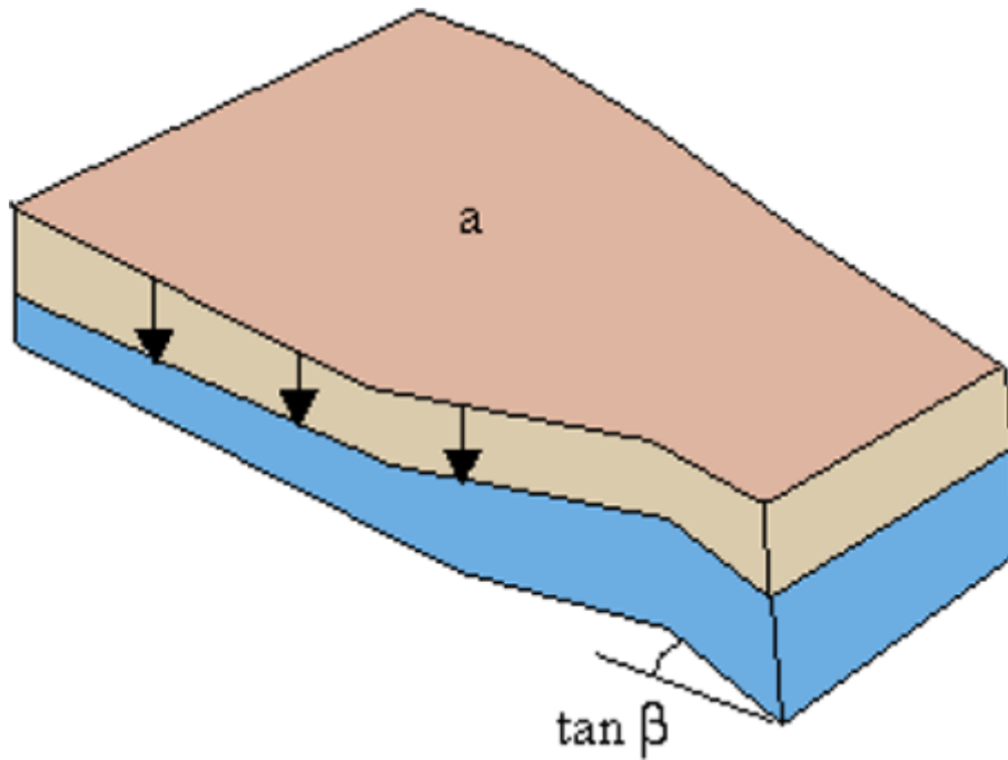
Fig. 3. Determination of the Kirkby's topographic index.
