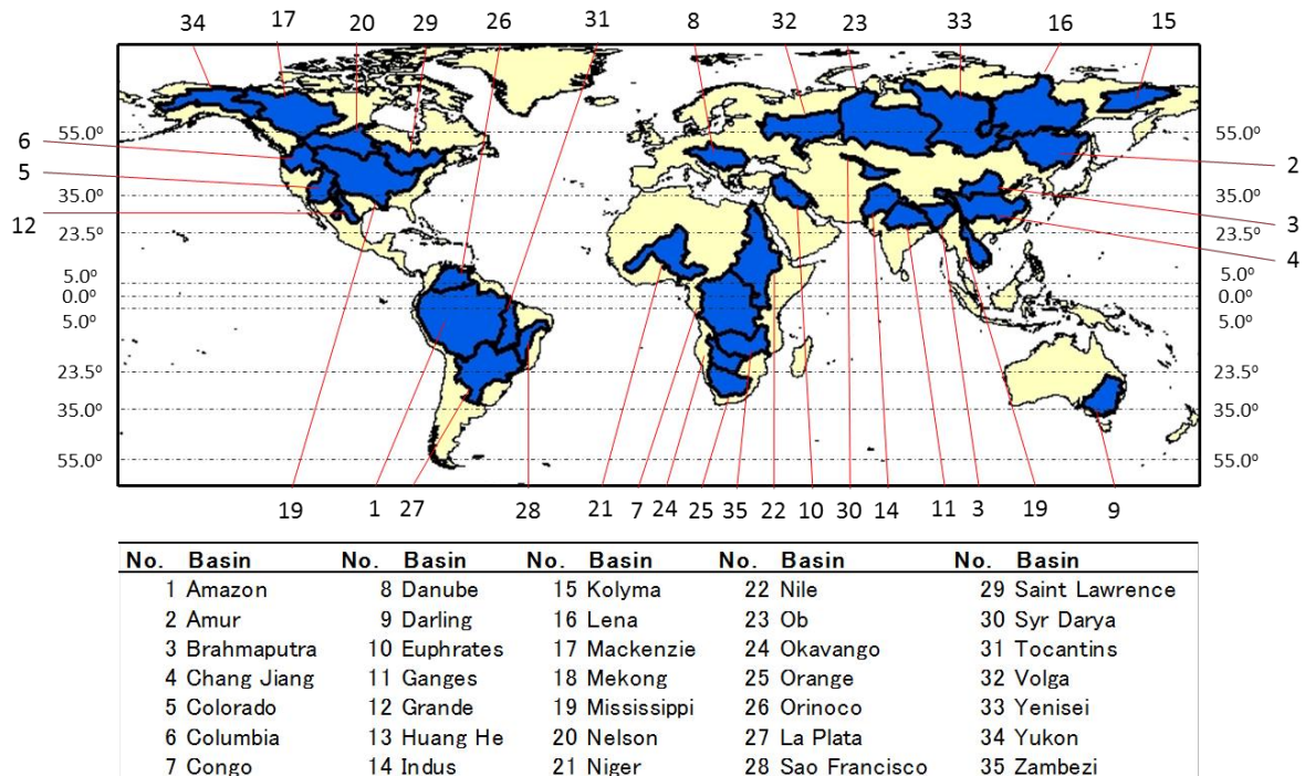
1 2 Figure 2. Location of the basins included in the analysis with an assigned identification 3 number. The latitude reference lines identify the latitudes that divide each of the regions 4 geographically separating the basins.
