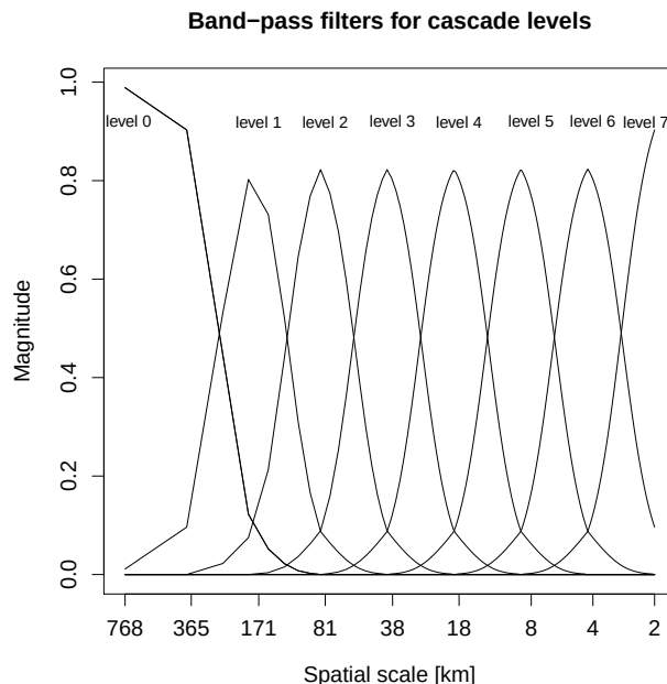
Figure 2. The set of 8 Gaussian band-pass filters used to isolate the spatial frequencies composing the cascade levels. The total magnitude for a given spatial frequency is normalized to one.
