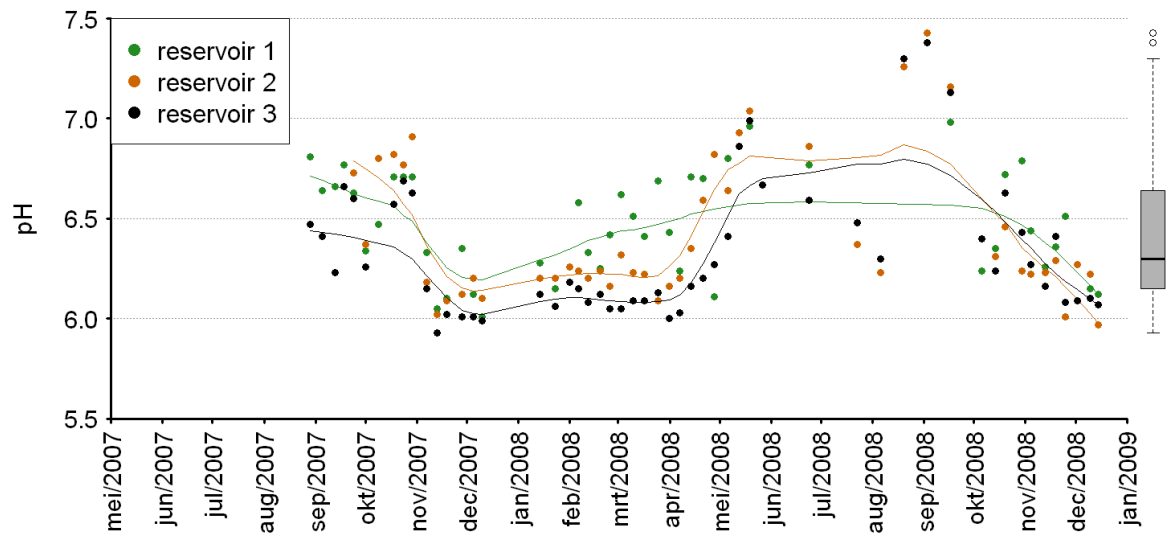
Figure 4. Time series of pH of reservoir water. Remarks as for Figure 2.
