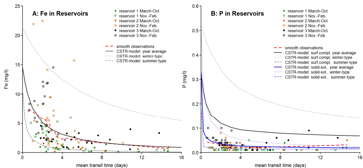
Figure 6. Measured Fe and P concentrations vs. the mean transit time of the water in the reservoirs. The blue and gray lines show the steady-state Fe and P concentrations according to the CSTR-models as function of the mean transit time for the yearly average situation ( T = 9.3^{\circ}\text{C} ; \text{pH} = 6.32 ; P_{\text{O}_2} = 0.21 ), the winter-type conditions ( T = 5^{\circ}\text{C} ; \text{pH} = 6.17 ; P_{\text{O}_2} = 0.21 \text{ atm.} ) and summer-type conditions ( T = 17^{\circ}\text{C} ; \text{pH} = 6.53 ; P_{\text{O}_2} = 0.1 \text{ atm.} ).
