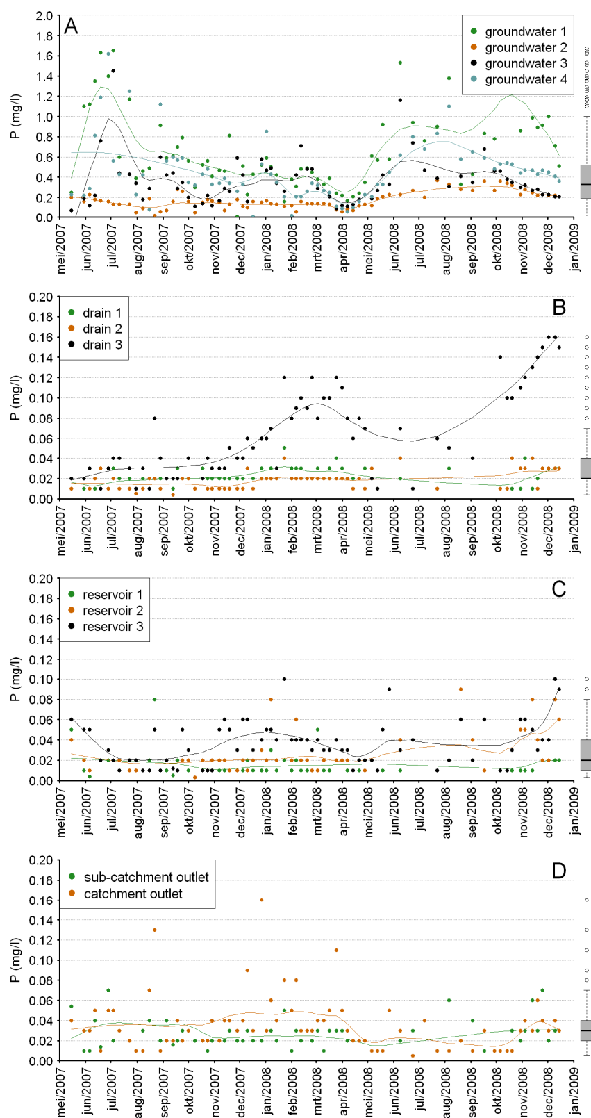
Figure 3. Time series and boxplots of dissolved total P concentrations of groundwater (A), tube drain water (B), in-stream reservoir water (C) and surface water (D). B, C and D share the same y-axis. Remarks as for Figure 2.
