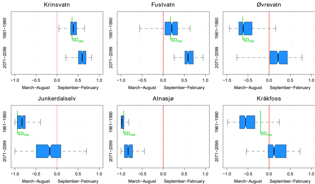
Figure 3. Boxplots showing the seasonality index S_D for all ensemble realizations for the reference and future period. The boxes show the interquartile of the values; the whiskers show the full range of the projections. The green bars in the upper panel of each plot ( SD_{obs} ) indicate the observed seasonality index S_D .
