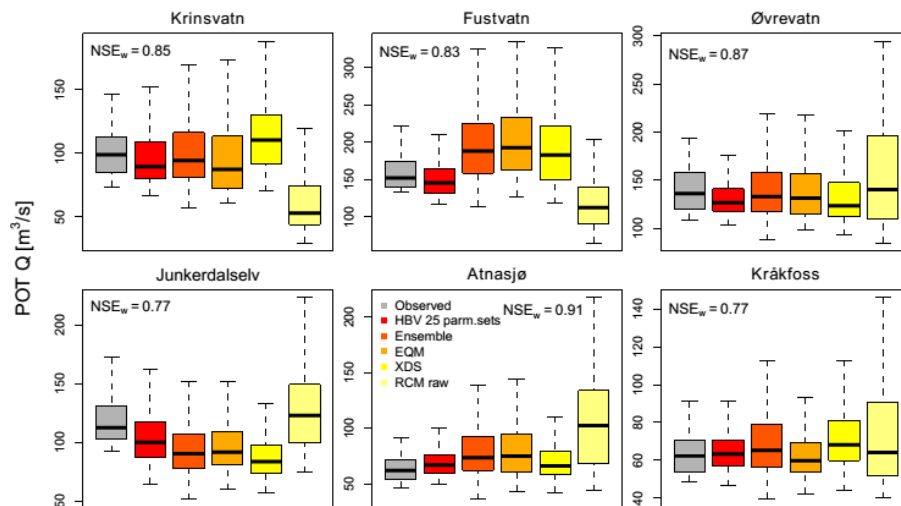
Figure 2. The distributions of POT events for the reference period from observed (grey) and simulated streamflow series generated by the calibrated HBV model using (from left to right panels): (i) observed climate data with the 25 best-fit parameter sets, (ii) the entire ensemble (i.e. all GCM/RCM combinations, LAMs, and hydrological parameter sets), (iii) the data locally adjusted by EQM, (iv) the data locally-adjusted by XDS, and (v) the raw RCM data. For the simulations (iii)–(v) only one best-fit HBV parameter set is considered.
