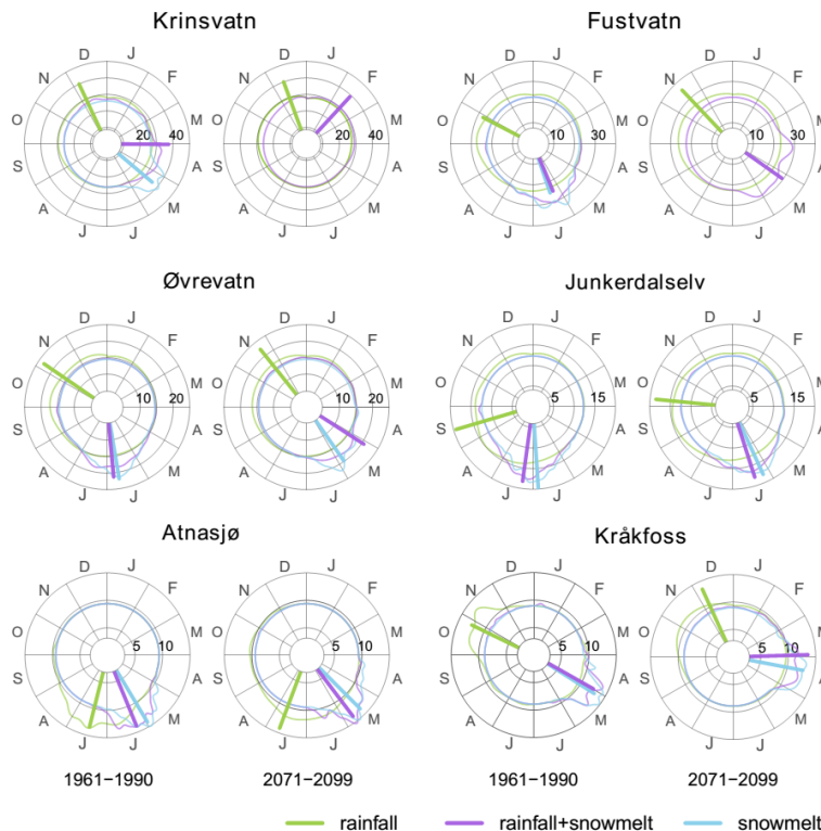
Figure 6. Circular plots showing (i) the circular kernel density function of the simulated POT events according to their FGPs [normalized; no units], and (ii) the median POT event magnitude [mm day -1 ] as bars according to their circular mean Julian date of occurrence and their FGPs for the reference and future period.
