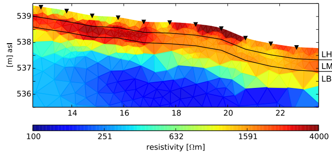
Figure 5. ERT section of profile A with plotted layer boundaries. (date: 21.10.08)
