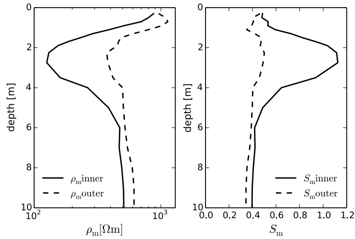
Figure 6. Median resistivity (left panel) and median water saturation (right panel) per depth for the inner region (between the depression lines) and outer region (hillslopes). (date: 21.10.08)
