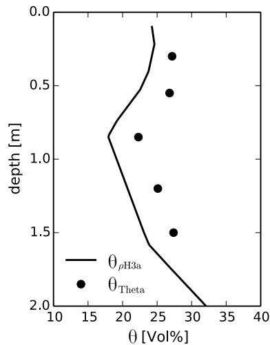
Figure 7. Volumetric water content calculated from resistivity data close to H3a in comparison with soil moisture sensors. (date: 21.10.08)
