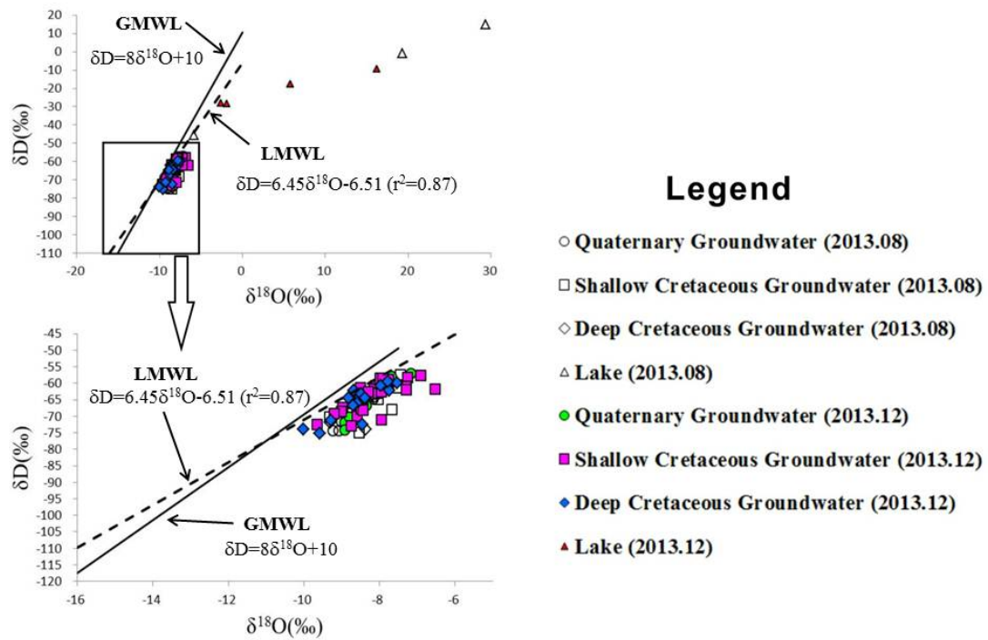
Fig.7 Relationship between hydrogen and oxygen isotopes in groundwater and lake water in August and December, 2013.
