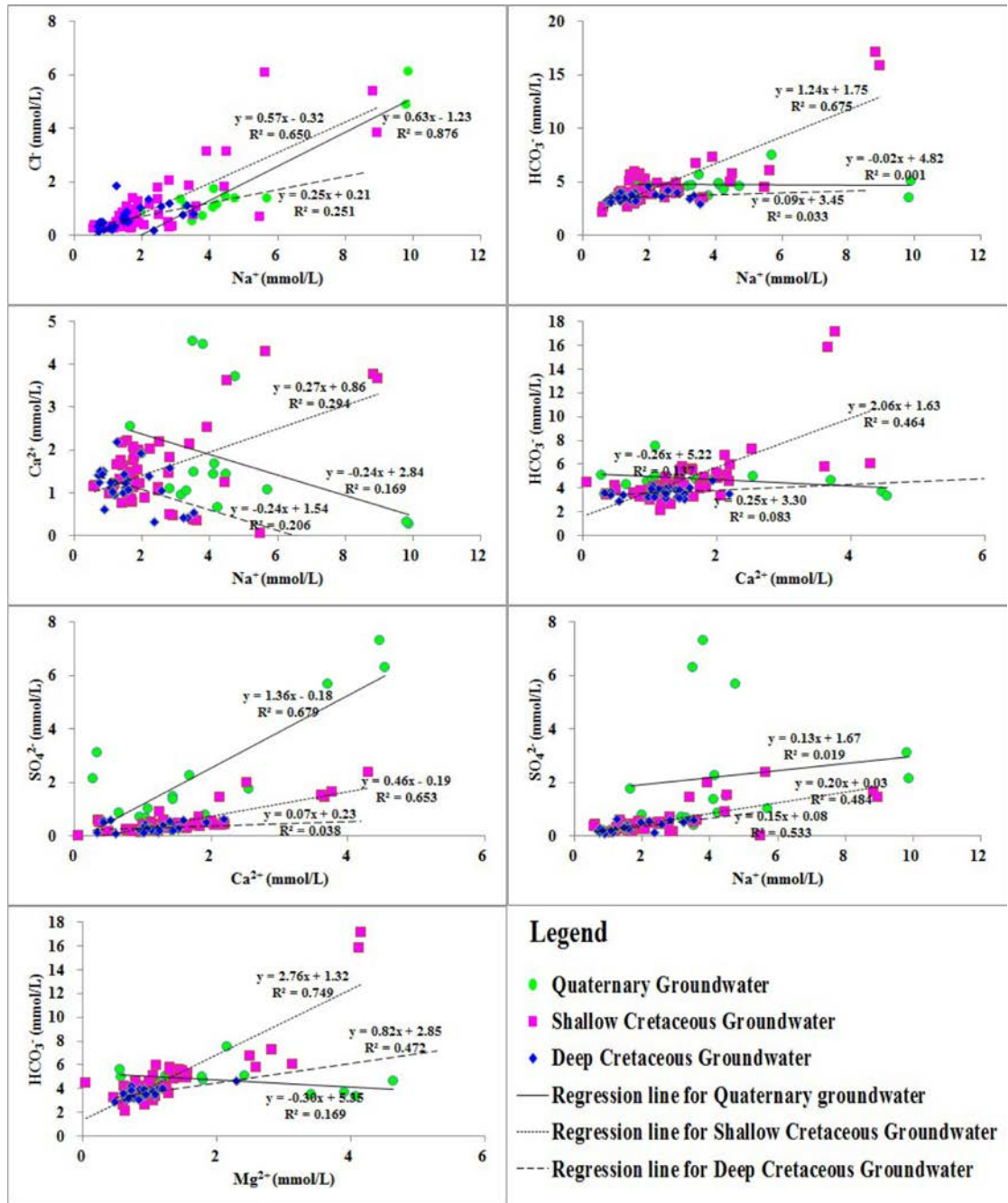
Fig.8 Relationship between some pairs of ions in groundwater.
