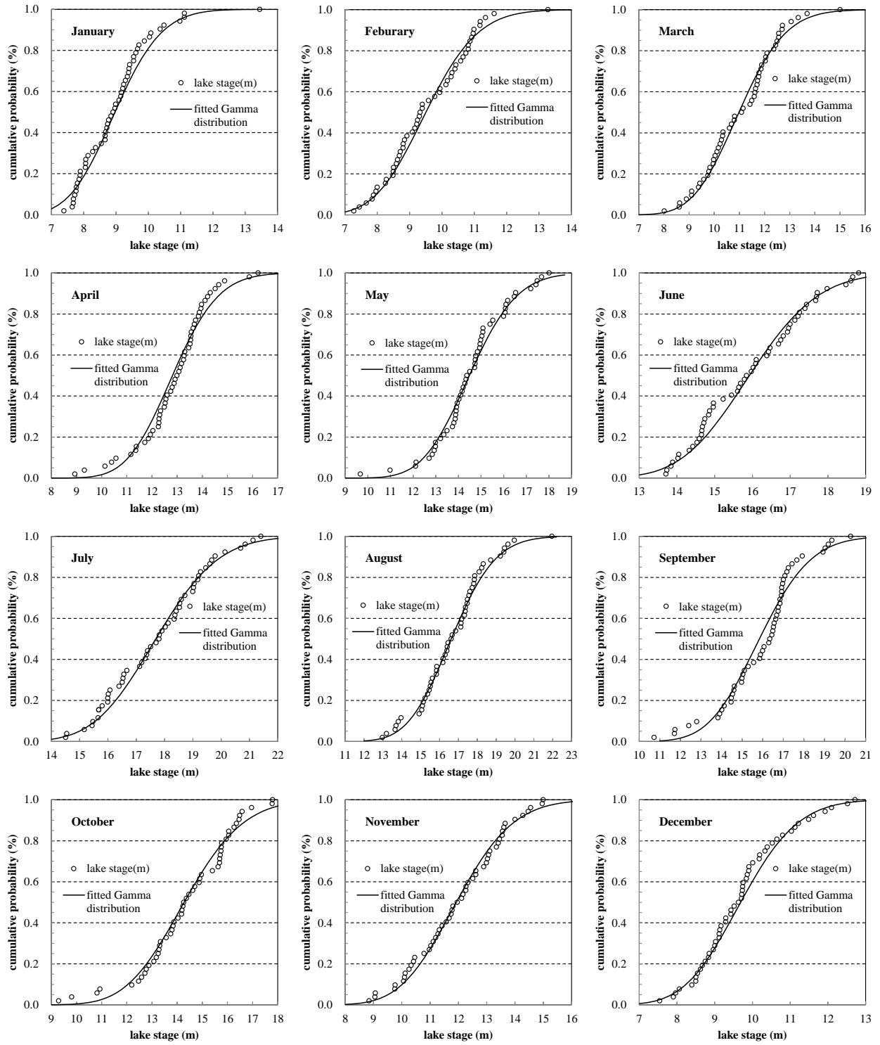
Figure 2. Statistical distribution of monthly average lake stages with a fitted Gamma distribution for each calendar month at Xingzi of Poyang Lake in 1961-2010.
