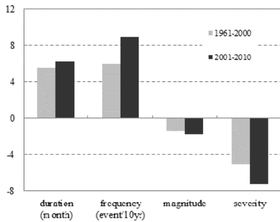
Figure 3. Poyang Lake droughts in 2001-2010. (a) Variation in standardized lake stage index (SLI). (b) Drought duration, frequency, magnitude and severity. Vertical axis indicates values for the four indices. (c) Drought frequency for moderate, severe and extreme droughts, compared to 1961-2000.
