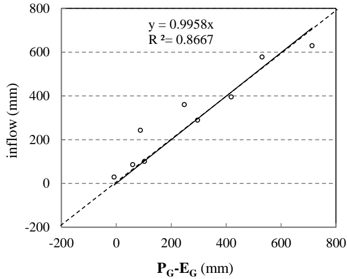
Figure 5. (a) Multi-year mean of monthly precipitation ( P_G ) and evapotranspiration ( E_G ) for the Poyang Lake Basin, and outflow ( O ) into the Yangtze River. (b) The relationship between P_G - E_G and inflow for nine cases of Poyang Lake droughts. All the water amounts are normalized to equivalent water height of the whole Poyang Lake Basin.
