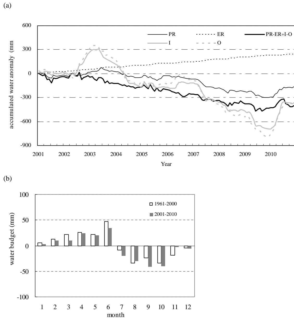
Figure 6. (a) Accumulated anomaly of water components and (b) water budget at the Poyang Lake region for 2001-2010 compared to 1961-2000. All the water amounts are normalized to equivalent water height of the whole Poyang Lake Basin.
