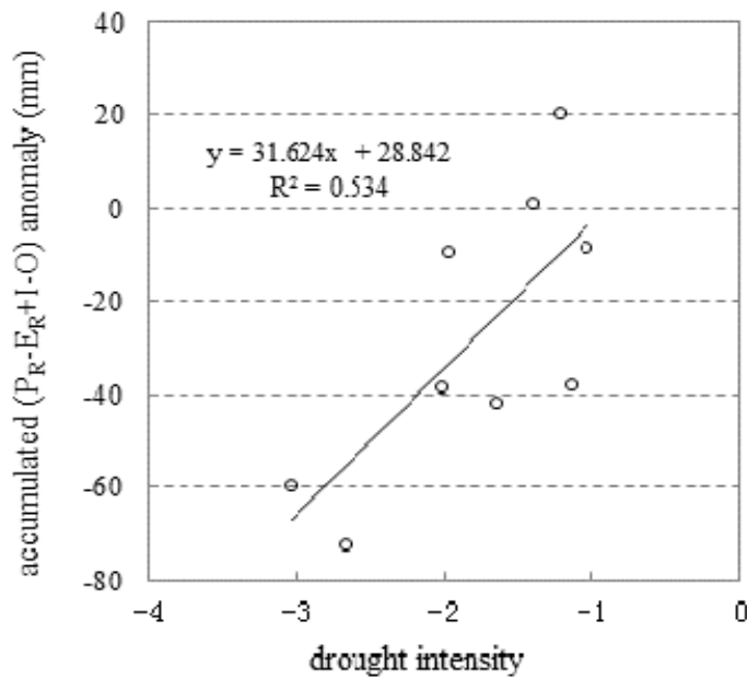
Figure 4 (a) Multi-year mean of monthly precipitation ( P_R ) and evapotranspiration ( E_R ) for the Poyang Lake region, lake inflow ( I ) from five major rivers of the Poyang Lake Basin, and outflow ( O ) into the Yangtze River. All the water amounts are normalized to equivalent water height of the whole Poyang Lake Basin. (b) The relationship between drought intensity and accumulated anomaly of (P_R - E_R + I) of each event for nice cases of Poyang Lake droughts.
