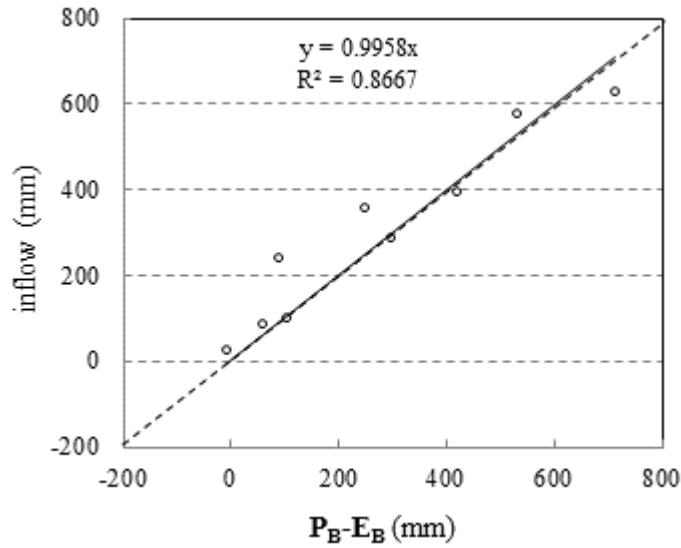
Figure 5. (a) Multi-year mean of monthly precipitation ( P_B ) and evapotranspiration ( E_B ) for the Poyang Lake Basin, and outflow ( O ) into the Yangtze River. (b) The relationship between P_B - E_B and inflow for nine cases of Poyang Lake droughts. All the water amounts are normalized to equivalent water height of the whole Poyang Lake Basin.
