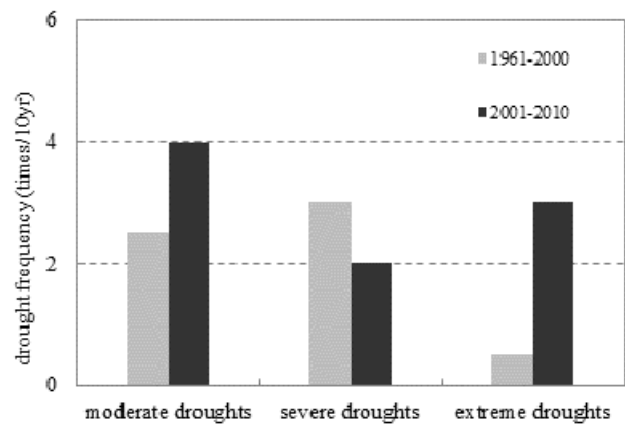
Figure 3. Poyang Lake droughts in 2001-2010. (a) Variation in standardized lake stage index (SLI). (b) Drought duration, frequency, magnitude and severity. Vertical axis indicates values for the four indices. (c) Drought frequency for moderate, severe and extreme droughts, compared to 1961-2000.
