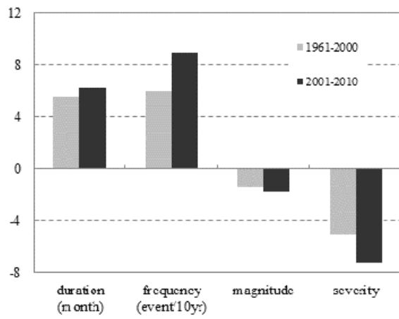
Figure 3. Poyang Lake droughts in 2001-2010. (a) Variation in standardized lake stage index (SLI). (b) Drought duration, frequency, magnitude and severity. Vertical axis indicates values for the four indices. (c) Drought frequency for moderate, severe and extreme droughts, compared to 1961-2000.
