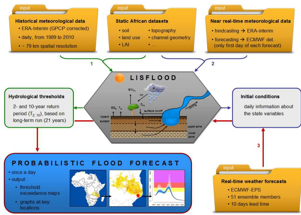
Figure 3. Schematic overview of AFFS.
