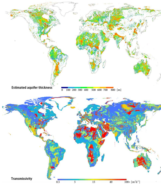
Fig. 3. Calculated aquifer thickness and transmissivities.
