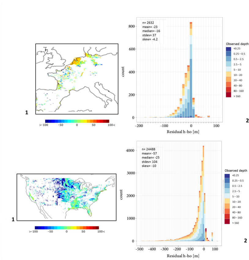
Fig. 7. Maps of residuals for NW-Europe and USA. (1) residuals and (2) histograms of residuals. Each bar in the histogram is clustered based on observed on classified groundwater depths.
