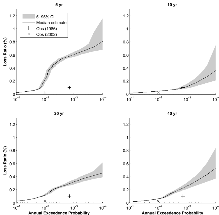
Fig. 7. Exceedence probability plots produced by the catastrophe model when trained using the gauge record cropped to four different lengths. The grey shaded area denotes the 5–95 % confidence intervals generated by the financial model. The losses simulated when the hydraulic and vulnerability models are driven with observed flows for two historical events are shown for reference.
