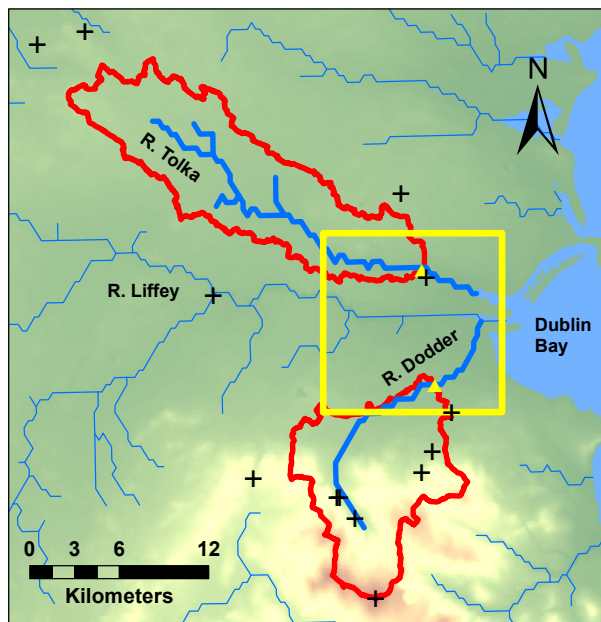
Fig. 1. Map of Dublin region. Modelled rivers are shown by thick blue lines. Hydrological model boundaries are shown in red. Hydraulic model boundary is shown in yellow. Rain gauge locations shown by black crosses. River flow gauges are shown by yellow triangles.
