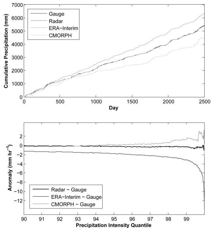
Fig. 6. Plots showing cumulative precipitation for each source (top) and anomalies in > 90th quantile precipitation intensities between gauge and other sources (bottom).
