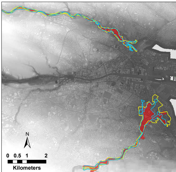
Fig. 3. Hydraulic model calibration results. Red shaded area shows observed flood extent. Blue outline shows flood outline from 10 m resolution model. Yellow outline shows flood outline from 50 m resolution model. Underlying DEM is 10 m resolution.
