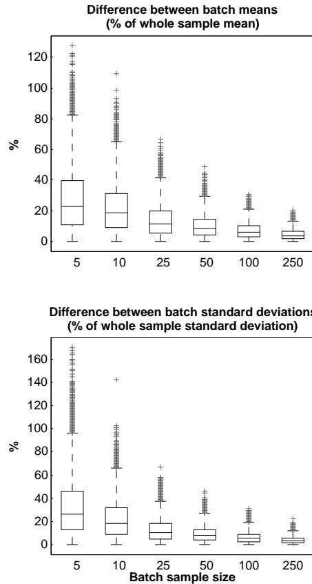
Fig. 4. Box plots that show the variation between two batches of simulations reducing as the number of simulations in each batch increases. The top plot shows the difference between the means of the two batches, expressed as a percentage of the mean loss across all 500 simulations. The bottom plot shows the difference between the standard deviations of the two batches, expressed as a percentage of the standard deviations across all 500 simulations.
