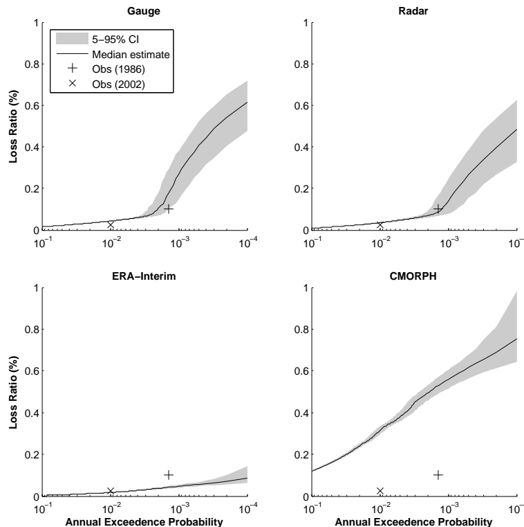
Fig. 5. Exceedence probability plots produced by the catastrophe model when trained using the four different precipitation datasets. The grey shaded area denotes the 5–95 % confidence intervals generated by the financial model. The losses simulated when the hydraulic and vulnerability models are driven with observed flows for two historical events are shown for reference.
