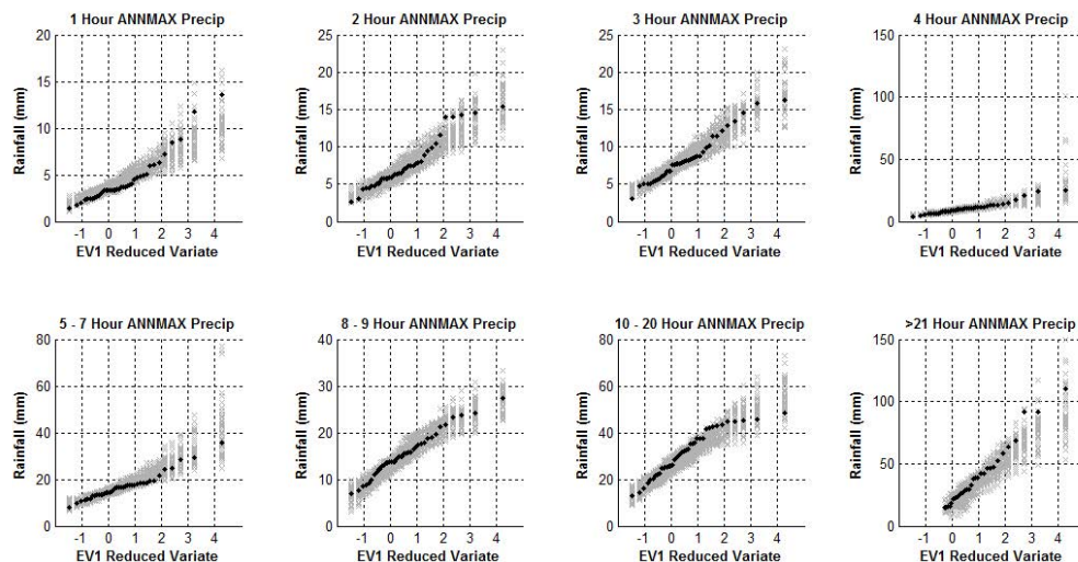
Fig. 2. Modelled annual maximum rainfall totals for each duration class compared to observational record. The annual maxima for each class in the 40 yr observed record are ranked and plotted using Gringorten plotting positions (black circles). The process was repeated for 50 \times 40 yr simulated series (grey crosses).
