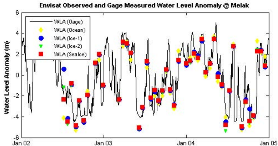
Fig. 8. Water level anomaly at Melak as observed by two Envisat passes and retracked by four retracers; compared with in-situ water level anomaly.
