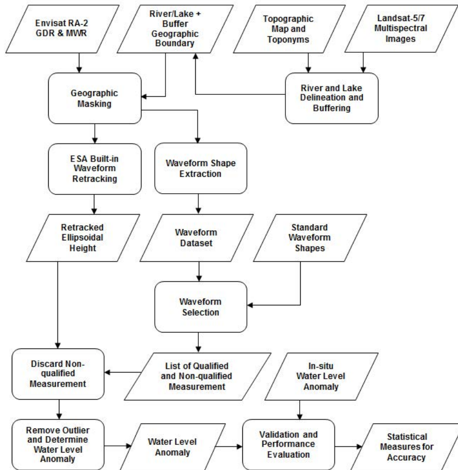
Fig. 4. Data processing workflow.
