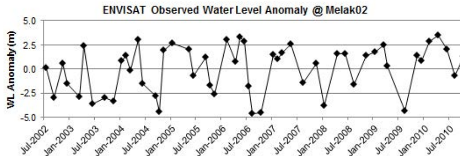
Fig. 7. ENVISAT Observed Water Level Anomaly at Site Melak02 (river width 294 m) as measured by Envisat RA-2 and processed by Ice-1 retracker.
