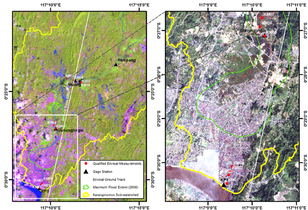
Fig. 11. Overview of Karangmumus Sub-watershed and Envisat ground track with background of Landsat-7 image of January 2007 (left) and IKONOS of February 2002 (right, in the extent of white box of the left image).
