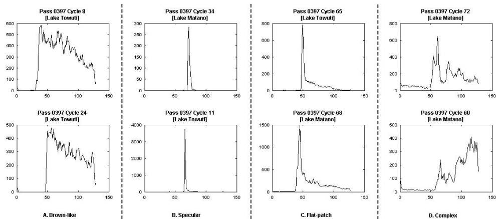
Fig. 3. General categories of waveform shapes.
