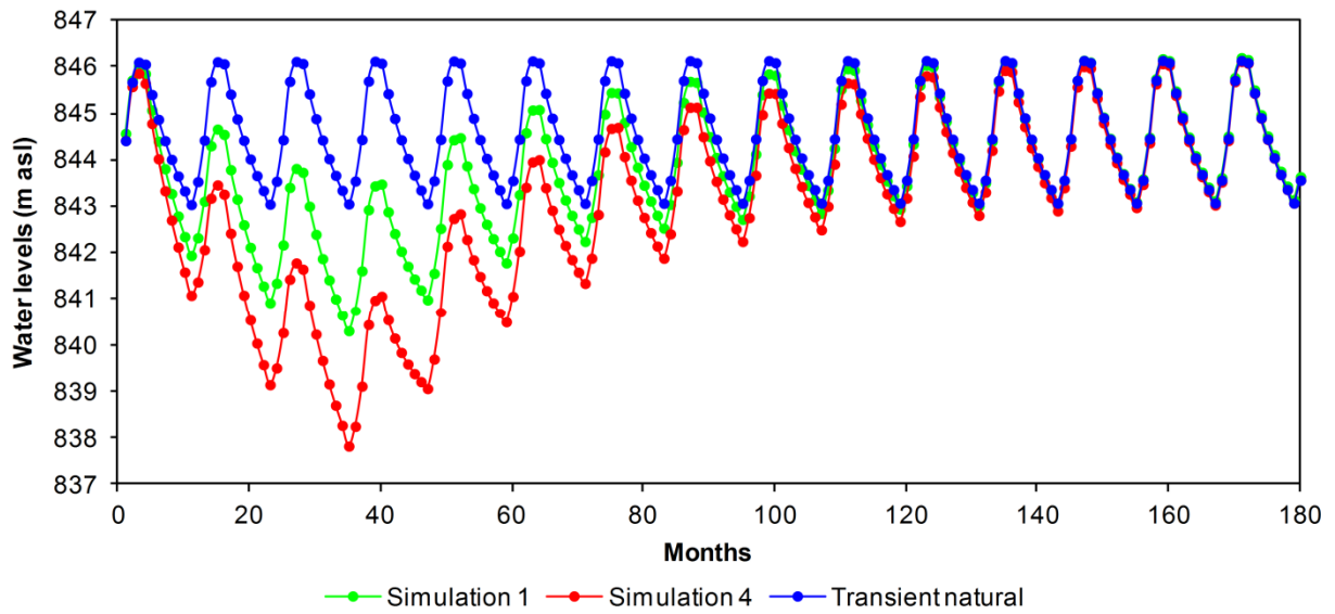
3 Figure 12 Simulated groundwater levels in well observation AC00232 at White river catchment
