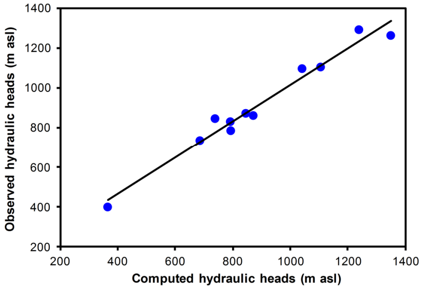
Figure 10 Scatter plot of the computed and observed groundwater heads
