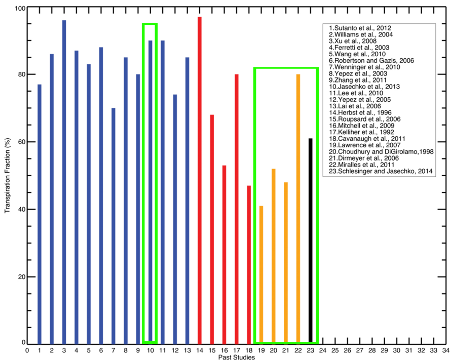
Fig. 1. Transpiration fraction from several past partitioning studies. The plot shows maximum values of transpiration fraction from those studies. Blue color is for isotope-based methods, red color is for hydrometric methods, orange is for global land surface model results, and black color is a combination hydrometric and model result. The studies inside the green boxes present global average values.
