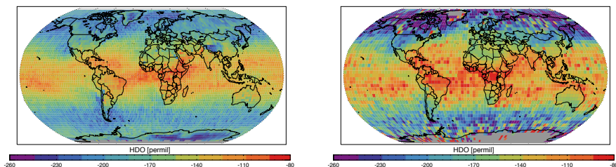
Fig. 3. Water vapor isotopic composition ( \delta D ) measured from TES (version 5 year 2006, weighted averaged from 900 to 425 hPa, left) and SCIAMACHY (average over 2003 to 2005, total column, right) satellites. Red colors indicate an enrichment in heavy isotopes and blue and purple colors indicate a depletion in heavy isotopes.
