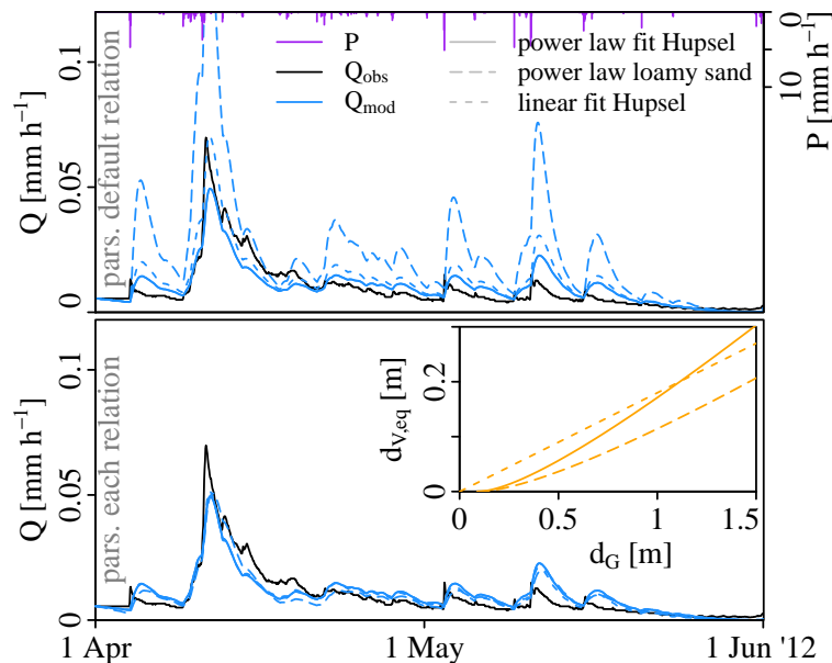
Fig. 14. Effect of the relation between groundwater depth and equilibrium storage deficit. Three options for this relation are plotted in the inset: the relation based on a power-law soil moisture profile (the default), fitted on soil moisture and groundwater observations in the Hupsel Brook catchment (solid; default), the relation based on the theoretical power-law soil moisture profile for loamy sand (long dashed; Brooks and Corey, 1964) and a linear fit between soil moisture and groundwater observations in the Hupsel Brook catchment (dashed).
