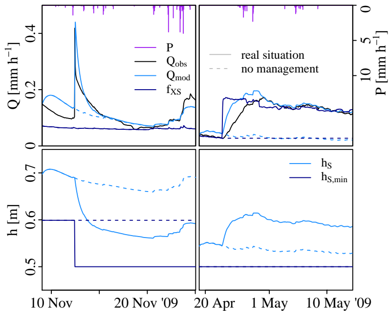
Fig. 10. Reproduction of the Cabauw polder response to water management interventions: weir level decrease (left panels) and increase in surface water supply (right).
