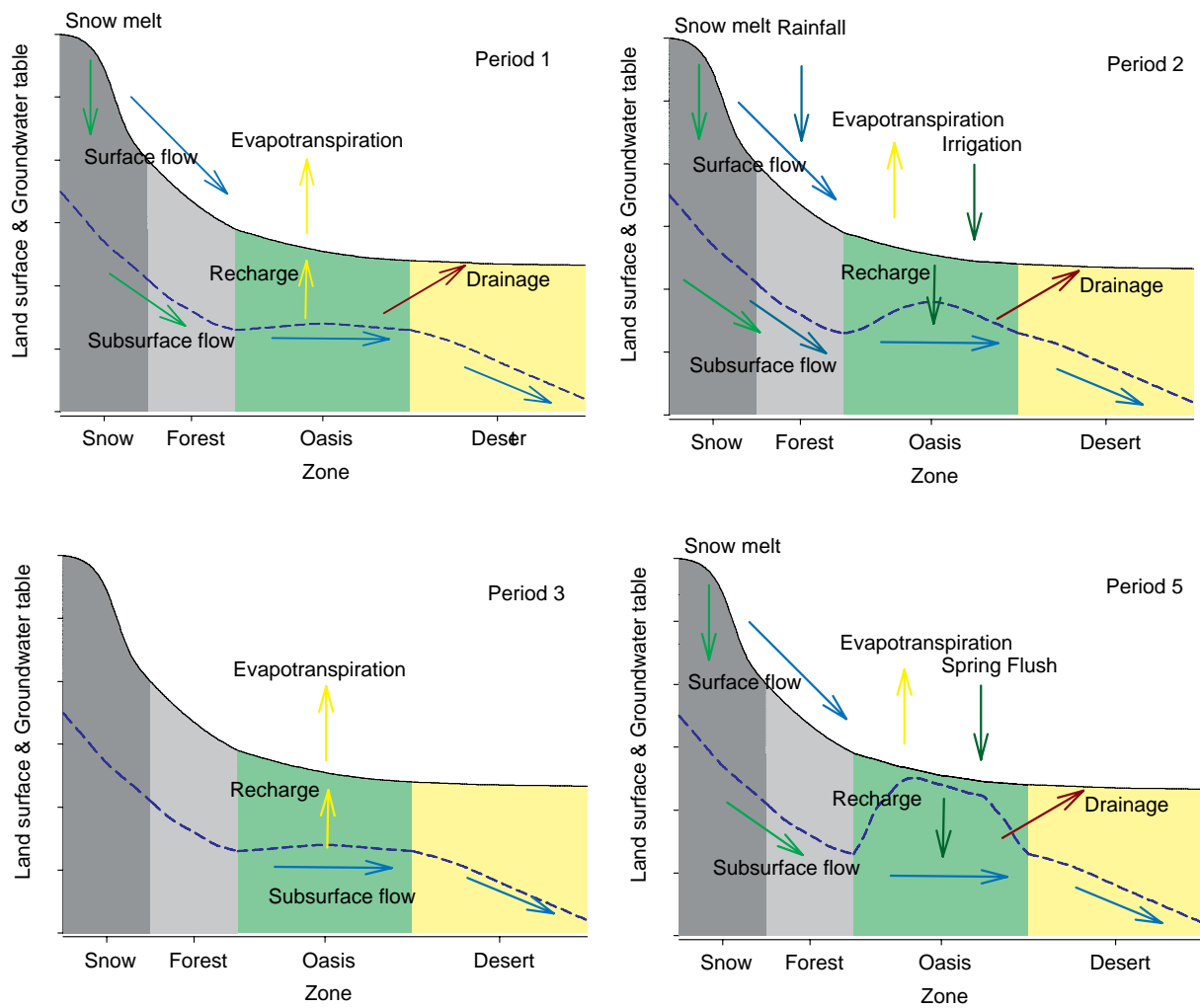
Fig.8 Sketch of seasonal groundwater dynamics (typical qualitative patterns in this region)
