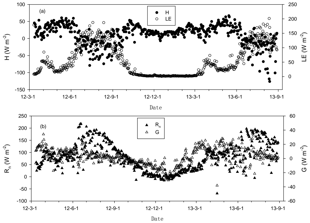
Fig.4 The daily variations in averaged sensible heat ( H ), latent heat ( LE ), net radiation ( R_n ) and soil heat flux ( G ) during 2012-2013
