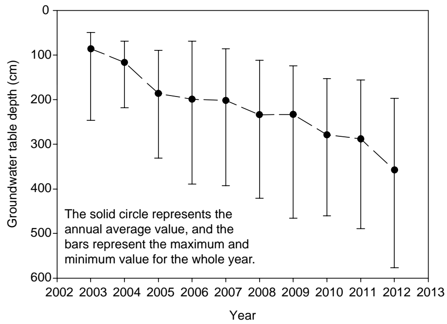
Fig.10 Long-term groundwater table variation in Yanqi County in KKRB
