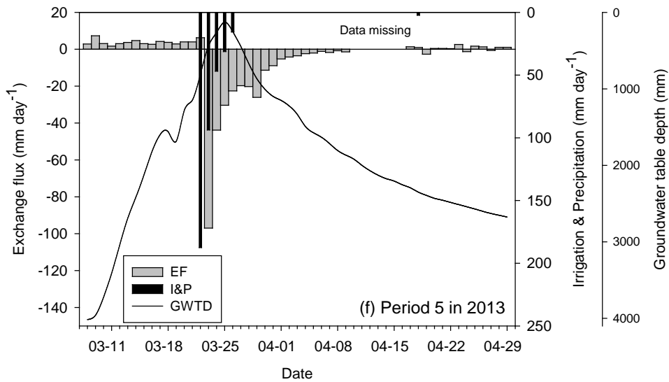
Fig.7 Exchange flux at 900 mm soil depth and groundwater table variation. Positive EFs represent upward fluxes and negative EFs represent downward fluxes.
