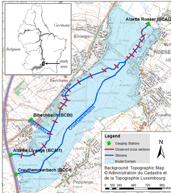
Fig. 1: Presentation of the study area and extension of the model domain
