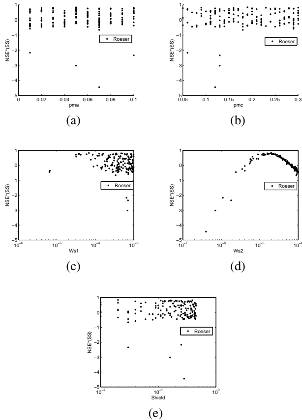
Fig. 5: Dotty plots of sediment transport model sensitivity analysis: evaluation of the simulated suspended sediment concentration according to (a) mud percentage in the Alzette riverbed ( p_{ma} ), (b) mud percentage in the Crauthembach riverbed ( p_{mc} ), (c) settling velocity of sand particles ( W_{s1} ), (d) settling velocity of mud particles ( W_{s2} ) and (e) critical Shields parameter ( \theta_c ).
