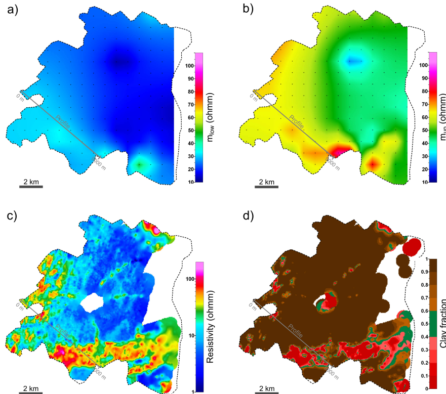
Fig. 7. Horizontal slices at 2 m b.s.l. cropped to the catchment area (dashed line). (a) The m_{\text{low}} parameters of the translator function superimposed with the 1 km translator function grid (black dots). (b) The m_{\text{up}} parameters of the translator function superimposed with the 1 km translator function grid (black dots). (c) Interpolated resistivity slice. (d) Resulting CF- model.
