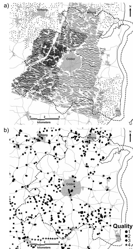
Fig. 4. (a) Location of the resistivity models. Small dots are SkyTEM models, larger scattered dots are ground-based models. (b) Borehole locations and borehole quality, where 1 corresponds to the highest quality and 4 to the lowest quality. The dashed line outlines the modeling area.
