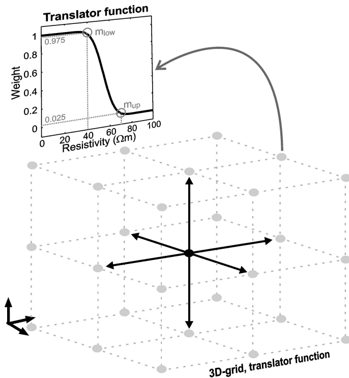
Fig. 2. The translator function and 3-D translator function grid. The translator function returns a weight, W , between 0 and 1 for a given resistivity value. The translator function is defined by the two parameters m_{low} , and m_{up} . In this example the the m_{low} , and m_{up} parameters correspond to 40 and 70 \Omega m respectively. Each node in the 3-D translator function grid holds a set of m_{up} and m_{low} . The m_{up} and m_{low} parameters are constrained to all neighboring parameters as indicated with the black arrows for the black center node.
