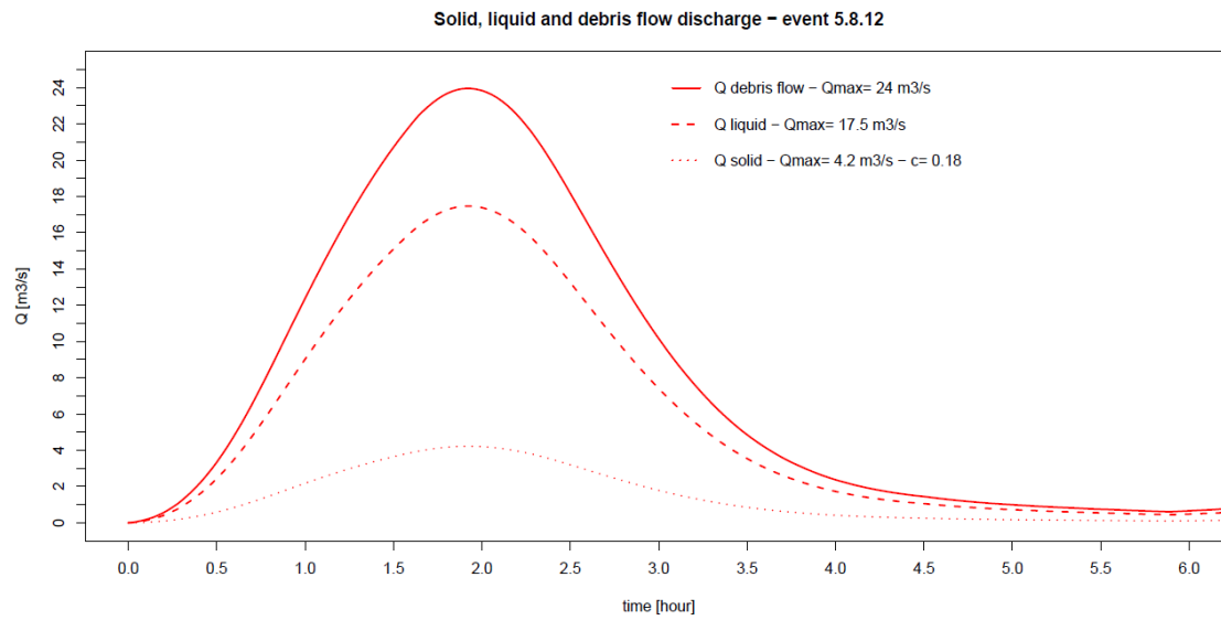
2 Figure 9. Boundary condition: input liquid, solid and mixture hydrograph.
