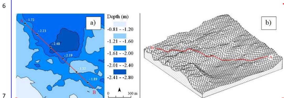
8 Figure 8. (a) Profile display, contour map. (b) Profile display, three-dimensional model
