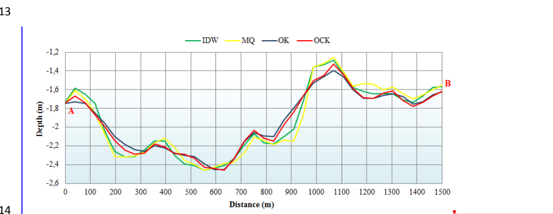
15 Figure 9. Differences in profile for the four best interpolation methods.
