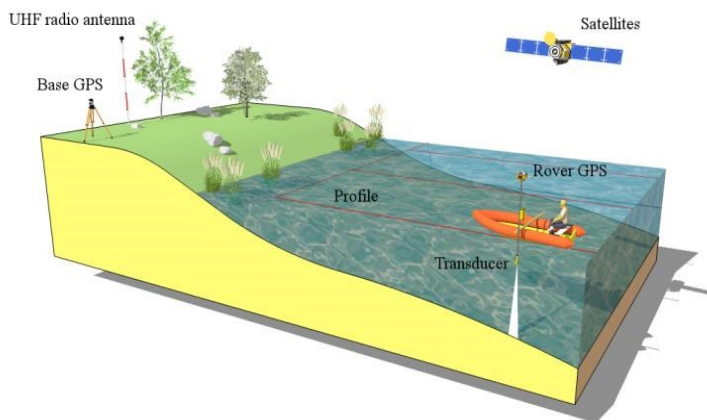
Figure 3. Integrated measuring system – combination of GPS-RTK and a sonar
