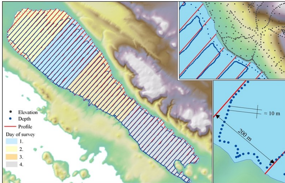
5 6 7 Figure 5. The phases and plan of the bathymetric survey
