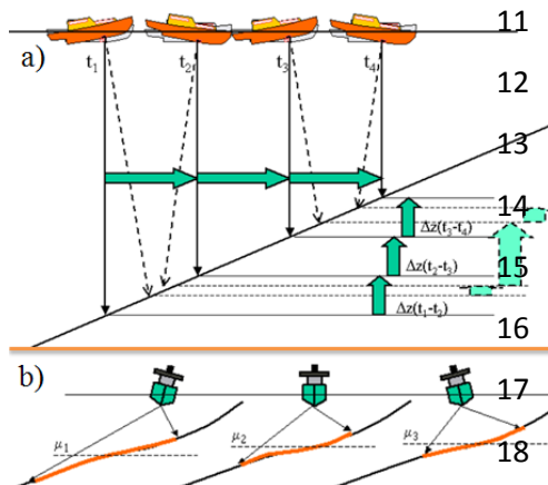
18 19 Figure 4. The effect of frontal (a) and dorsal (b) waves on data registration (Clarke, 2003).
