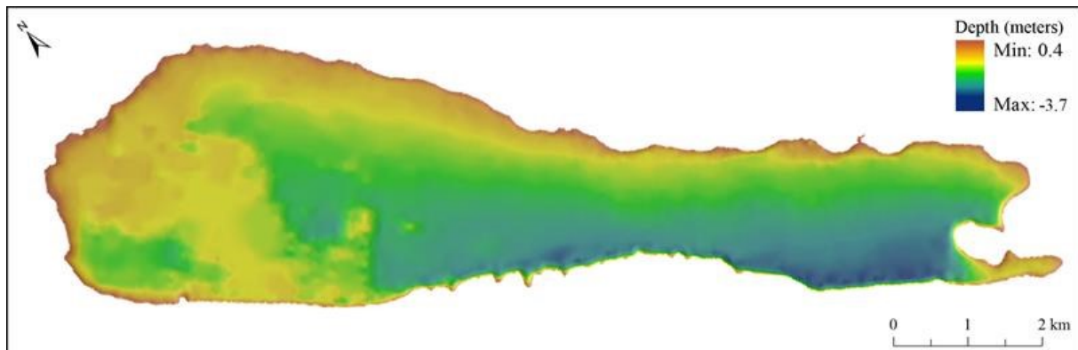
15 Figure 13. Bathymetric map of Lake Vrana (ordinary cokriging)
