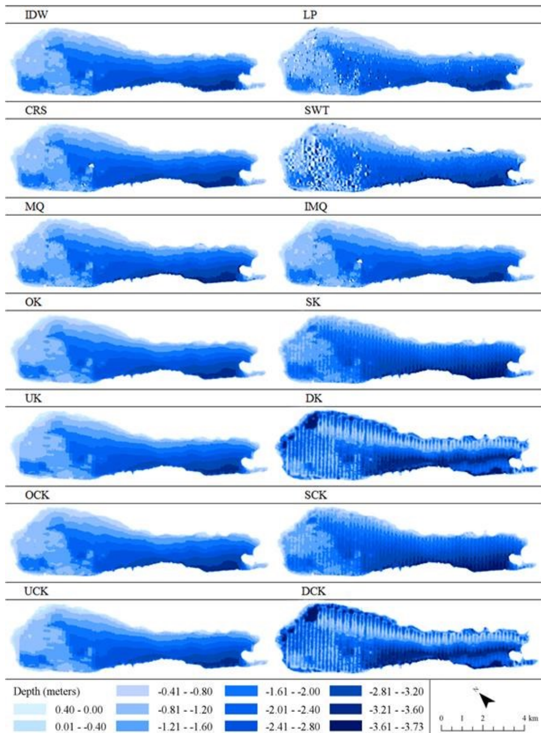
4 5 6 Figure 7. Digital elevation models generated from surveyed data, showing differences 7 between deterministic and geostatistical interpolation methods
