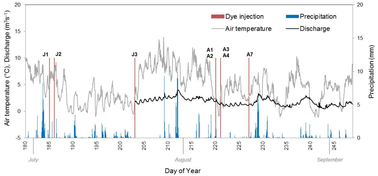
Figure 3. Measured 2 m air temperature, precipitation and proglacial discharge (calculated from relative gauging height) during summer 2013 (data illustrated spans 29th June – 5 th September). Values are plotted at hourly intervals where temperature and discharge are averages, and precipitation is a total. The timing of successful glacier-based dye injections are indicated in red.
