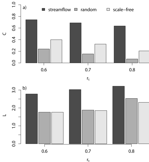
Figure 6. Change in the network clustering coefficient, C , and the average shortest path length, L , for the streamflow network for three values of the correlation coefficient threshold, r_t . Values for the equivalent random and scale-free networks are shown for reference (see Fig. 5 caption).
