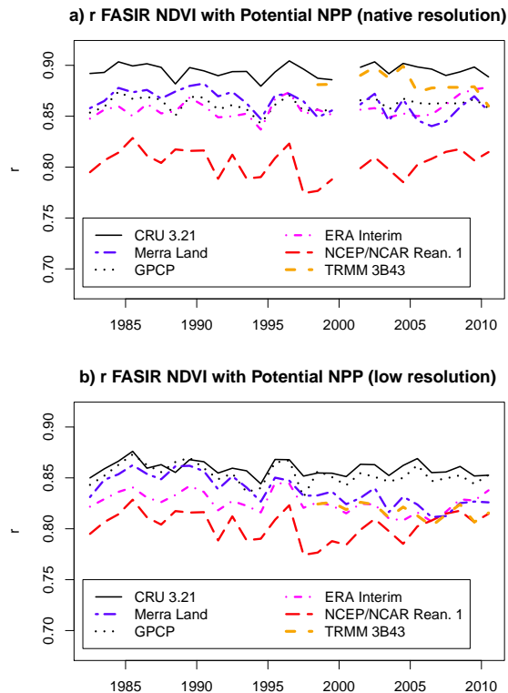
Figure 3. Spatial correlation for 1982–2010 between mean annual FASIR NDVI and potential annual NPP for 6 precipitation products. Correlations are calculated for the entire land surface between 45^{\circ} S and 45^{\circ} N and indicate spatial agreement between rainfall patterns and the vegetation index. Highest correlations are found for CRU NPP; lowest for MERRA (not MERRA Land) NPP (between 0.611 < r < 0.681 ; not shown). (a) Correlations at native resolution of precipitation data. (b) Correlations with data scaled to NCEP/NCAR resolution ( 1.875^{\circ} \times 1.875^{\circ} ).
