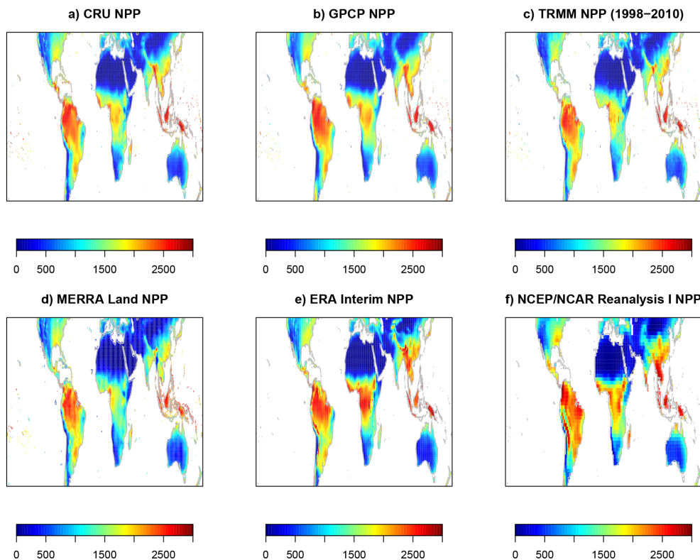
Figure 2. Spatial distribution of mean potential rainfall limited NPP fields derived from Lieth's model (Fig. 1). (a) Mean annual precipitation limited NPP for 1982–2010 from CRU data. (b) NPP for GPCP data, (c) NPP for TRMM 3B43 data, average is calculated over 1998–2010, (d) NPP for MERRA Land reanalysis, (e) NPP for ERA Interim reanalysis and (f) NPP for NCEP/NCAR Reanalysis I.
