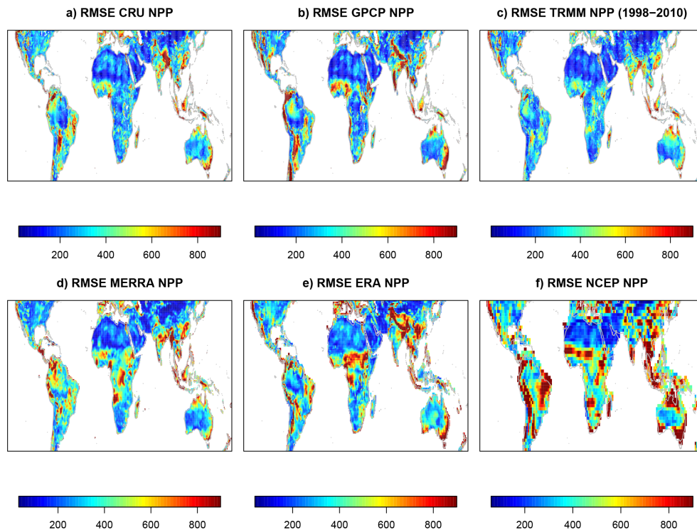
Figure 5. Root mean square error ( E_{\text{RMS}} ) from the model \text{NPP}_p - (\beta_1 \text{NDVI}) for the years 1982–1999 and 2000–2010. (a) CRU data (b) GPCP data, (c) TRMM data (d) MERRA Land reanalysis (showing larger E_{\text{RMS}} throughout) (e) ERA Interim reanalysis showing a large E_{\text{RMS}} south of the Sahara (f) NCEP/NCAR reanalysis.
