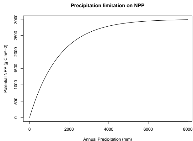
Figure 1. Lieth's Net Primary Production (NPP) model describing potential NPP ( \text{g C m}^{-2} \text{y}^{-1} ) as a function of annual precipitation. This model, as used in the present study, ignores other environmental limitations caused by, e.g., temperatures, soil properties, and solar radiation.
