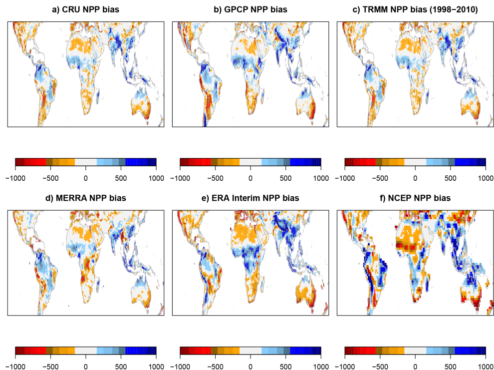
Figure 4. Mean deviation (bias) from the model NPP_p - (\beta_1 NDVI) for the years 1982–1999 and 2001–2010. (a) CRU data (b) GPCP data, (c) TRMM data (1998–2010 only) (d) MERRA Land reanalysis (e) ERA Interim reanalysis and (f) NCEP/NCAR reanalysis. The ERA Interim shows a large positive bias for tropical regions in Africa compared to the CRU and GPCP but patterns for other continents are similar. The NCEP/NCAR reanalysis shows a consistently larger bias than the CRU and GPCP data for most vegetated areas.
