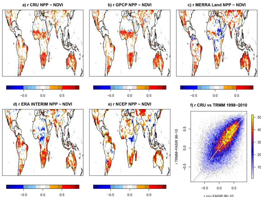
Figure 6. Spatial distributions of correlations (significant at p < 0.1 ) between NDVI time series and potential NPP time series calculated from annual precipitation amounts for 1982–2010 (2000 excluded). (a) Correlations for CRU data; (b) GPCP data (c) MERRA Land reanalysis (d) ERA Interim Reanalysis and (e) NCEP/NCAR reanalysis. (f) Density scatter plot of correlations for the CRU and TRMM data for the period of 1998 and 2010 (all correlations included; grey line is 1 : 1 line). All reanalysis products (c–e) show poor correlations for the Sahel and Savanna regions south of the Sahara. Notice areas with negative correlations in the South eastern parts of the Sahara in the CRU (a) and GPCP (b) data (see also Fig. 7).
