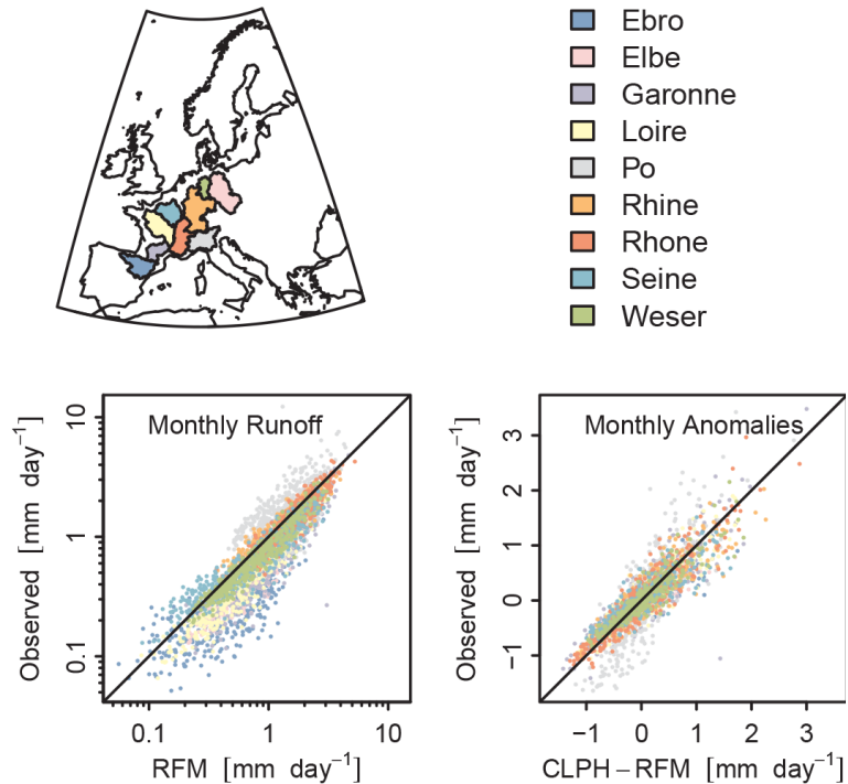
Figure 8. Basin scale validation: top, nine continental scale river basins used for model validation. Bottom, comparison between observed monthly river discharge to river discharge estimates derived from the Random Forest Model with full atmospheric forcing (left panel) and comparison between observed and modelled monthly discharge anomalies (right panel).
