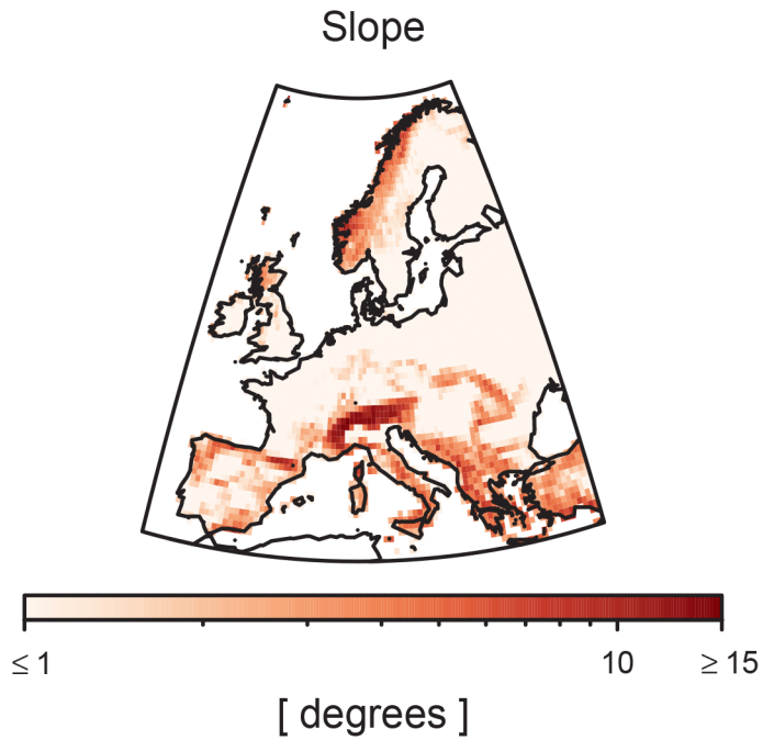
Figure 2. Median grid-cell slope.
