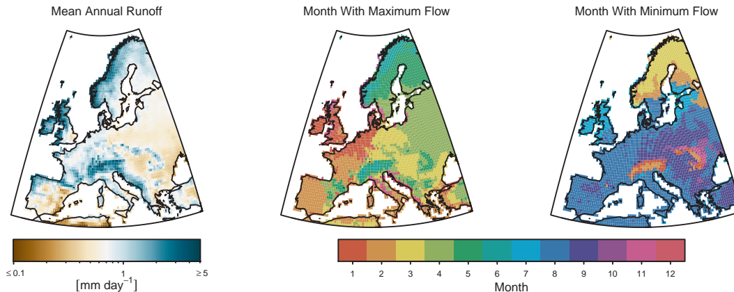
Figure 12. European runoff climatology (1964–2000): left panel: long-term mean daily runoff rates. Centre panel: maximum month of the long-term mean annual cycle. Right panel: minimum month of the long-term mean annual cycle.
