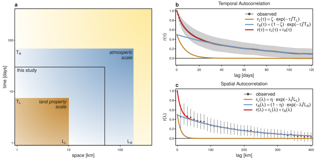
Figure 13. Time and space scales of runoff in Europe: (a) empirical results suggest that runoff in Europe has two space and time scales. A small scale ( T_L : time scale; L_L : space scale), at which runoff dynamics is strongly influenced by locally varying land properties, and a large scale ( T_A : time scale; L_A : space scale) at which runoff dynamics is dominated by atmospheric forcing. Both the spatial and temporal resolution of this study are located well above the scales at which land properties are expected to have a strong influence on runoff dynamics. (b, c) Small and large scales are estimated from observed autocorrelations of daily runoff anomalies in Europe. Vertical bars denote the SD of the observed autocorrelation. See text for details.
