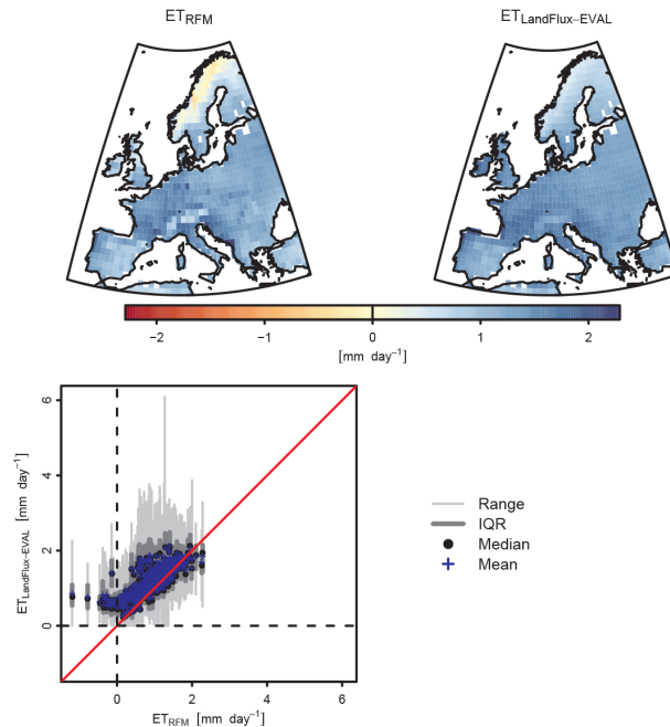
Figure 10. Comparison of mean evapotranspiration (1989–1995) derived from the Random Forest Model with full atmospheric forcing and the LandFlux-EVAL synthesis product: top left: mean evapotranspiration computed as the mean difference between precipitation and runoff derived from the RFM. Top right: mean evapotranspiration from the LandFlux-Eval synthesis product (Mueller et al., 2013). Bottom: comparison of the RFM and the LandFlux-EVAL estimates of mean evapotranspiration. The vertical bars denote the interquartile range (IQR) and the range of all 40 data sets entering the LandFlux-EVAL product. The points and crosses indicate the median and mean evapotranspiration of the LandFlux-EVAL product.
