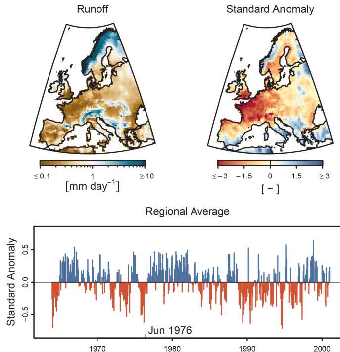
Figure 11. The 1976 drought in Europe: the top left panel shows the monthly runoff rate in June 1976. The top right panels shows the corresponding standardised runoff anomalies. The bottom panel shows the time series of the spatial average of standardised runoff anomalies for the entire region under investigation.
