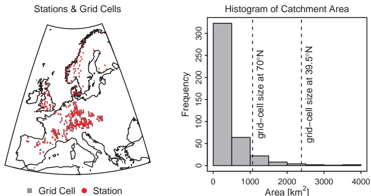
Figure 1. Runoff observations: left panel: locations of the gauging stations of the considered catchments, as well as the grid cells with observations. Right panel: histogram of catchment areas. The vertical lines indicate the grid-cell size of the southern- and northernmost grid cells.
