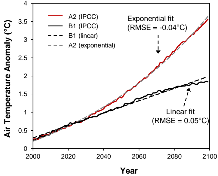
2 Figure 2: IPCC Multi-model globally averaged air temperature anomaly projections for 3 the 21 st century relative to the air temperature data for 1980-1999 for emission scenarios 4 B1 and A2 (data from, IPCC, 2007). Details concerning the exponential and linear fits to the 5 IPCC projections are given in Section 3.3.1. Modified from Kurylyk and MacQuarrie (2014).
