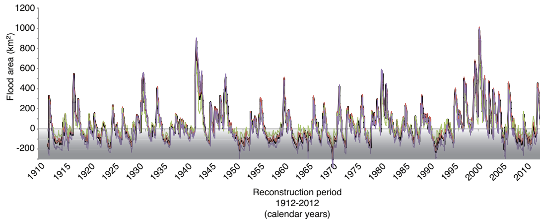
“ Figure A3: Surface water extent ( F_A ) at the Fortescue Marsh reconstructed using the final model based on the full 1988-2012 calibration period (black line) and the subsets for the 1998-2012 (red line) 1988-1997; 2005-2012 (green line), 1988-2004 (purple line) periods; F_A \leq 0 \text{ km}^2 = no surface water evident on the Marsh (shaded).”
