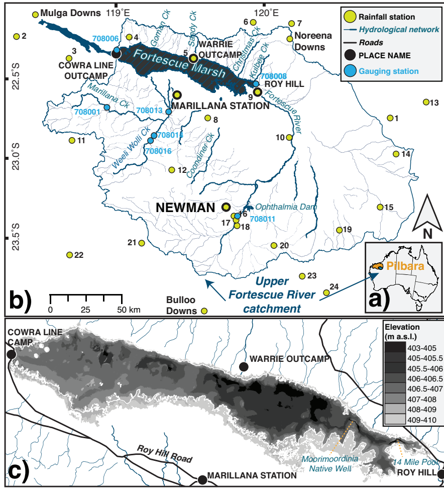
1 2 3 Figure 1: The a) Pilbara region in northwest Australia, b) Upper Fortescue River 4 catchment and river network (blue lines; DoW, 2014), including the Fortescue Marsh's 5 floodplain area used in this study (black hatched section; < 410 m a.s.l. extracted from a 6 sec DEM-H, Geoscience Australia, 2011), stream gauging stations (blue circles, see full 7 list in Appendix A, Table A1; WIN, 2014) and meteorological stations (green circles, see 8 full list in Appendix A, Table A2; www.bom.gov.au/climate/data/ ) and c) elevation of the 9 study area (0.1 m vertical accuracy (RMS) LiDAR Survey DEM; Fortescue Metals Group 10 Ltd, 2010) with roads and place name (black lines and circles; Geoscience Australia, 11 2001). Generated in ArcMap v. 9.2.
